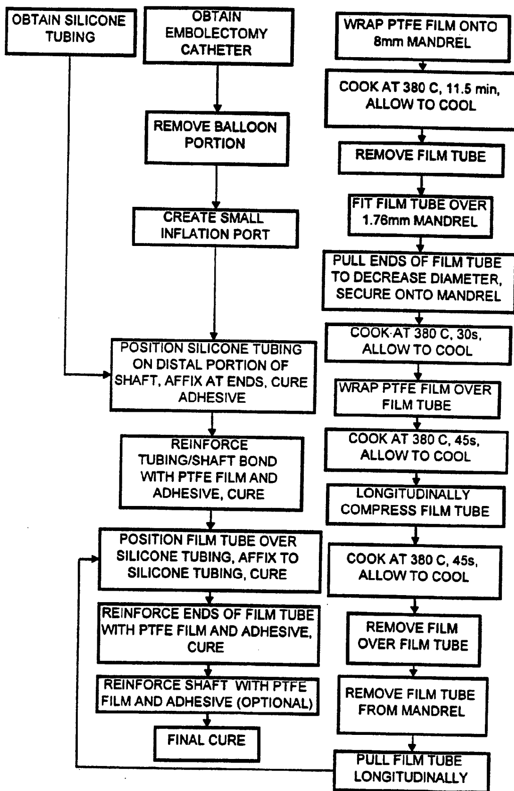
FIGURE 11C: EXAMPLE 8 FLOW CHART
