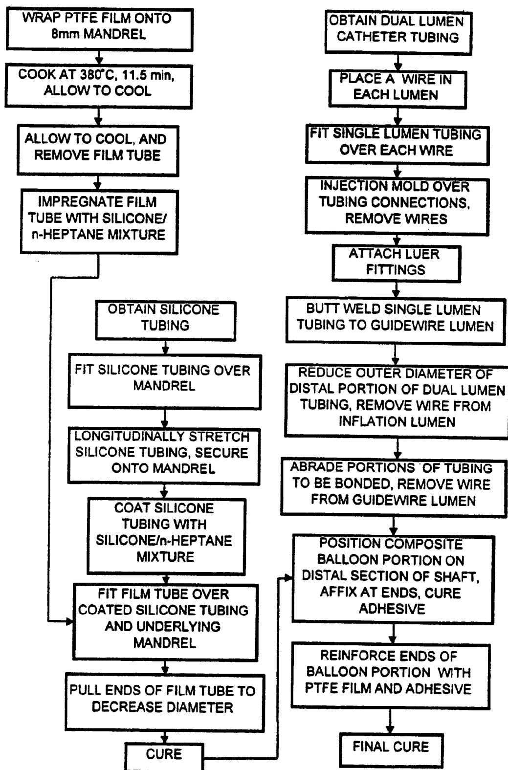
FIGURE 12C: EXAMPLE 9 FLOW CHART
