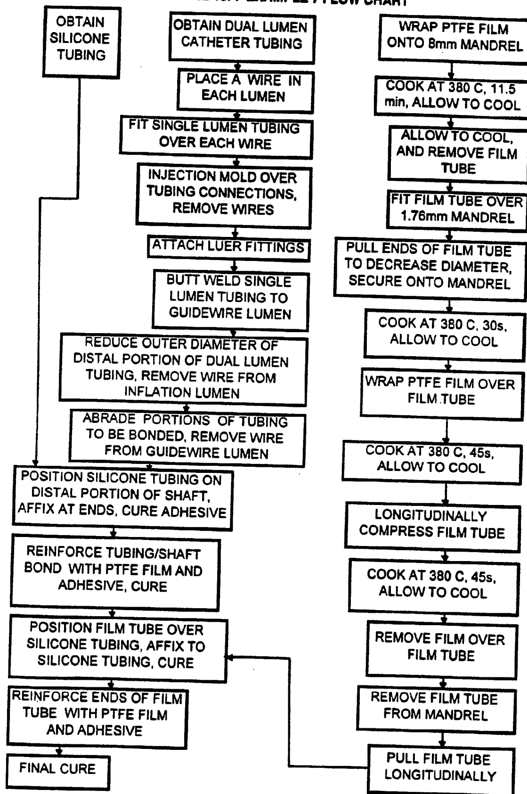
FIGURE 10F: EXAMPLE 7 FLOW CHART
