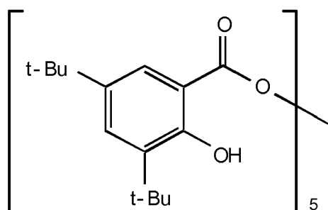
\text{Zr}_4\text{O}_4(\text{OH})_3 Structural Formula of aromatic oxycarboxylic acid metal compound 3
