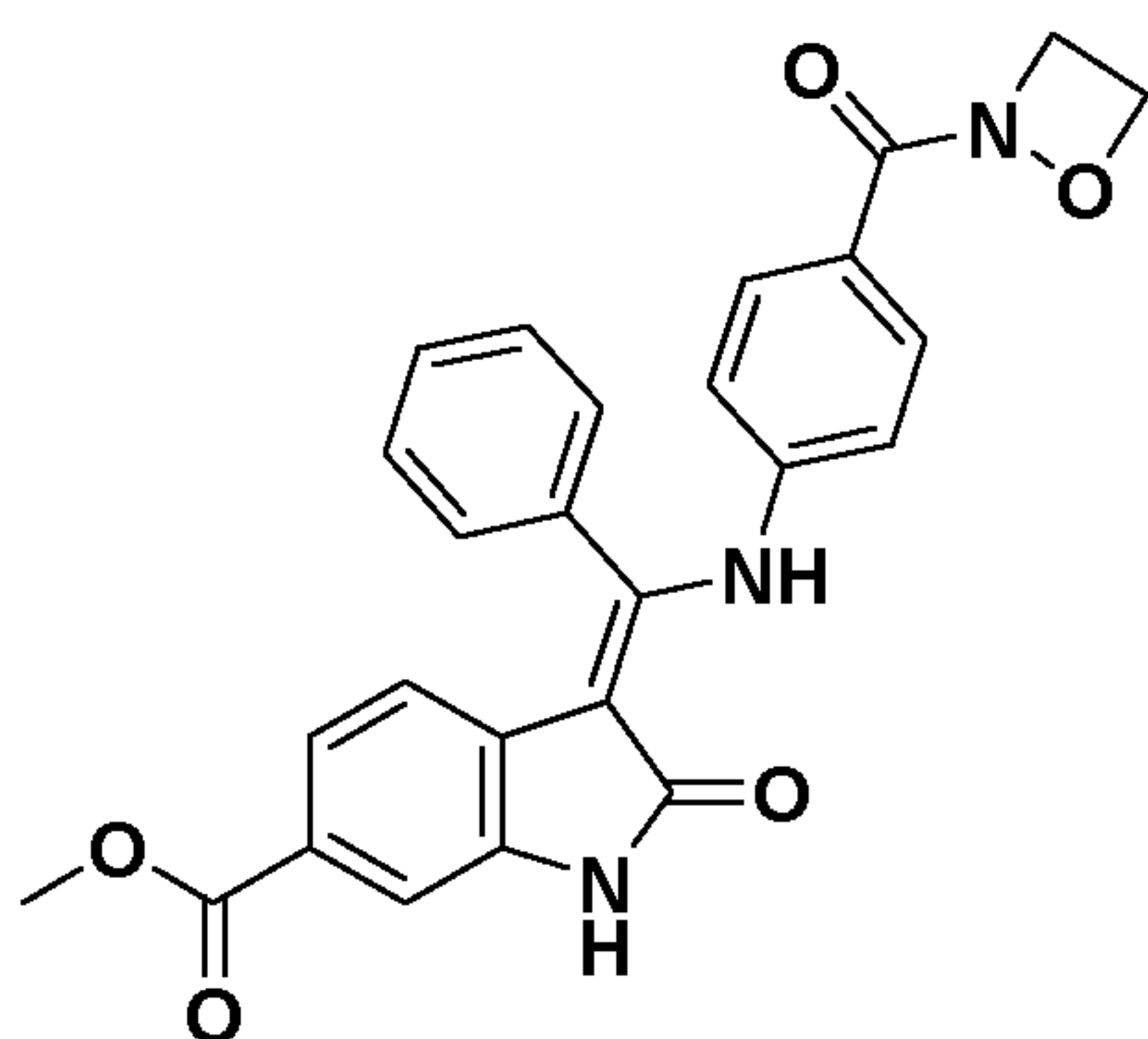
(Z)-Methyl 3-(((4-(1,2-oxazetidine-2-carbonyl)phenyl)amino)(phenyl)methylene)-2-oxoindoline-6-carboxylate
