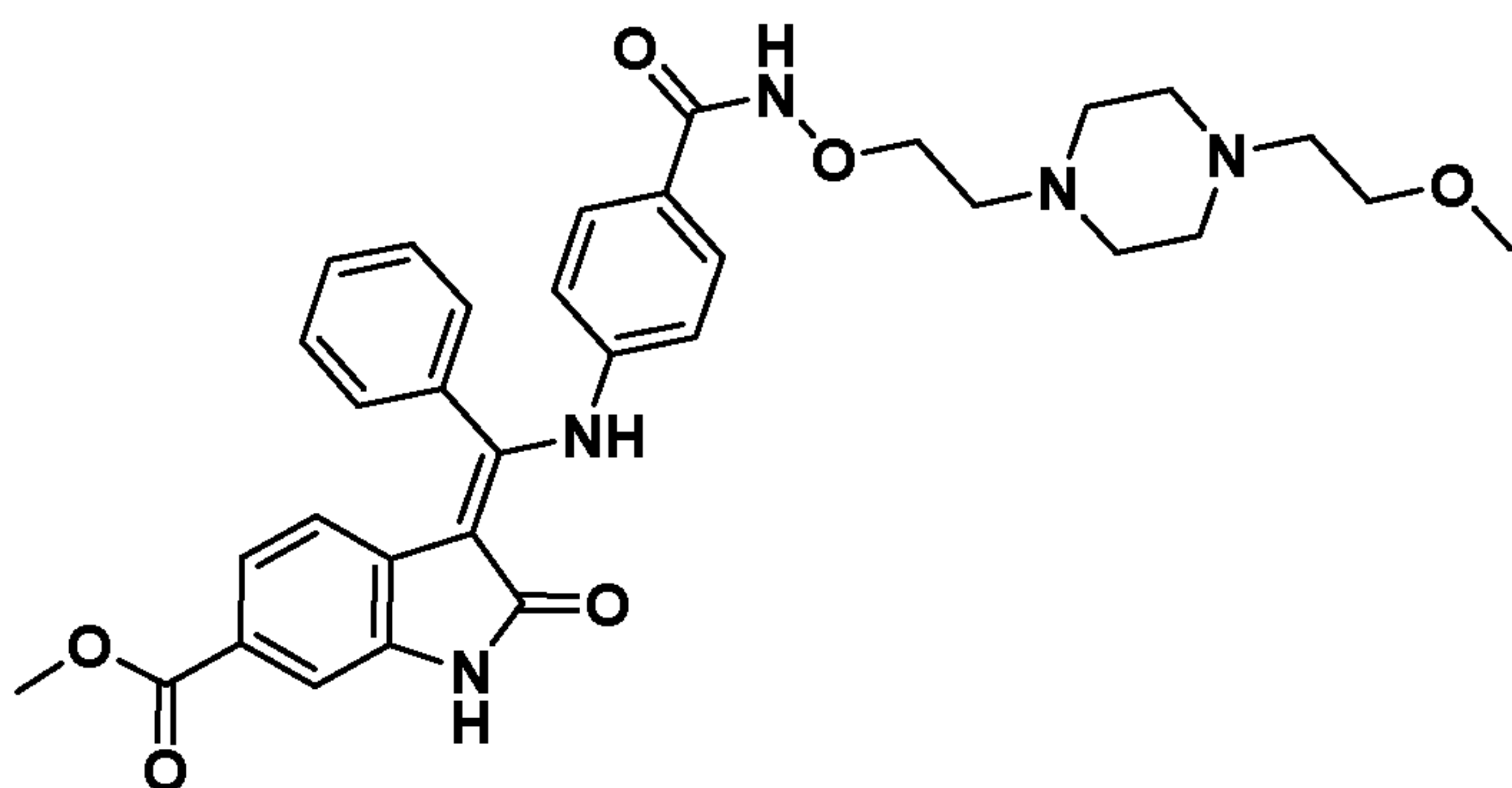
(Z)-Methyl 3-(((4-((2-(4-(2-methoxyethyl)piperazin-1-yl)ethoxy)carbamoyl)phenyl)amino)(phenyl)methylene)-2-oxoindoline-6-carboxylate, formate
