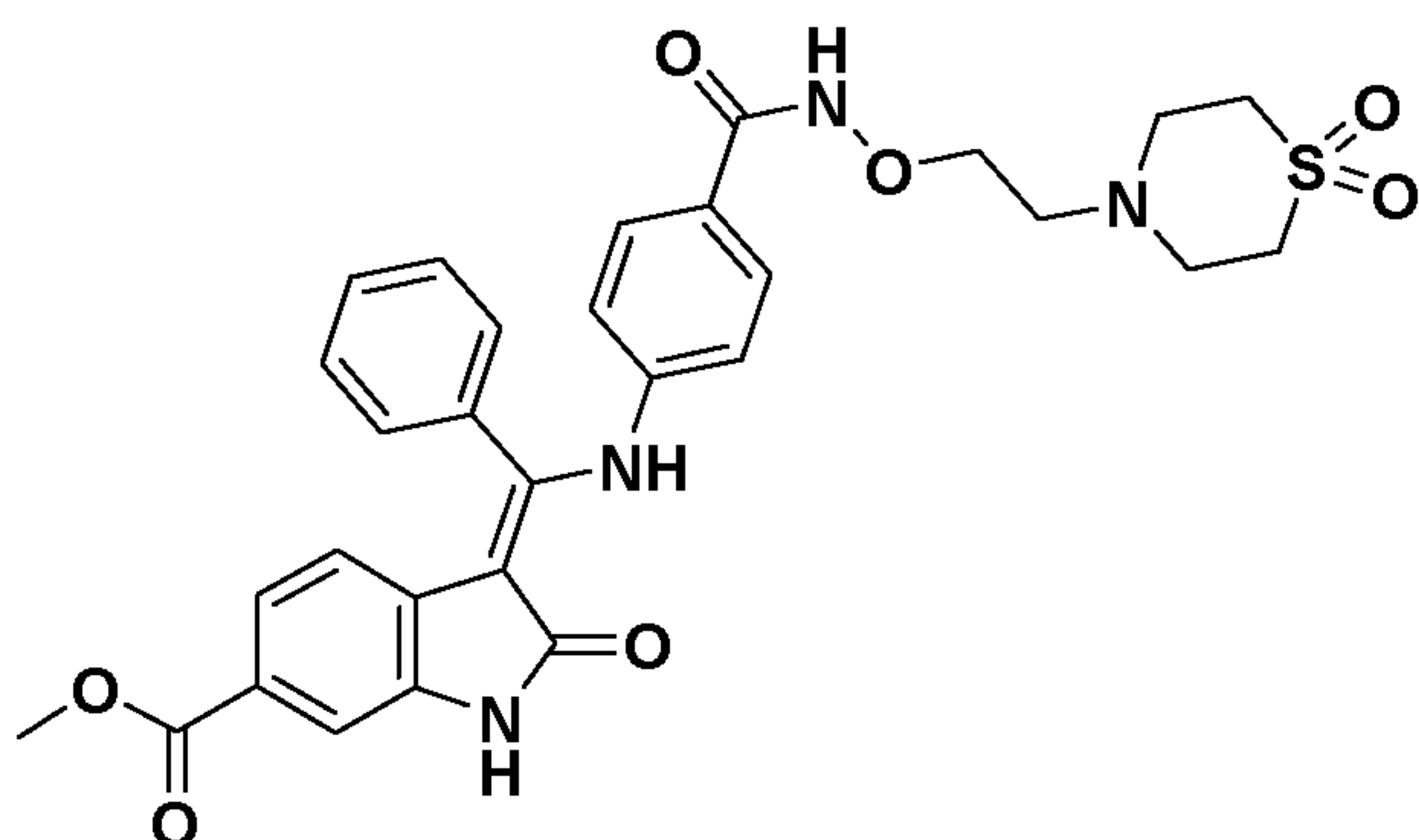
(Z)-Methyl 3-(((4-((2-(1,1-dioxidothiomorpholino)ethoxy)carbamoyl)phenyl)amino)(phenyl)methylene)-2-oxoindoline-6-carboxylate Route code*: 1C
