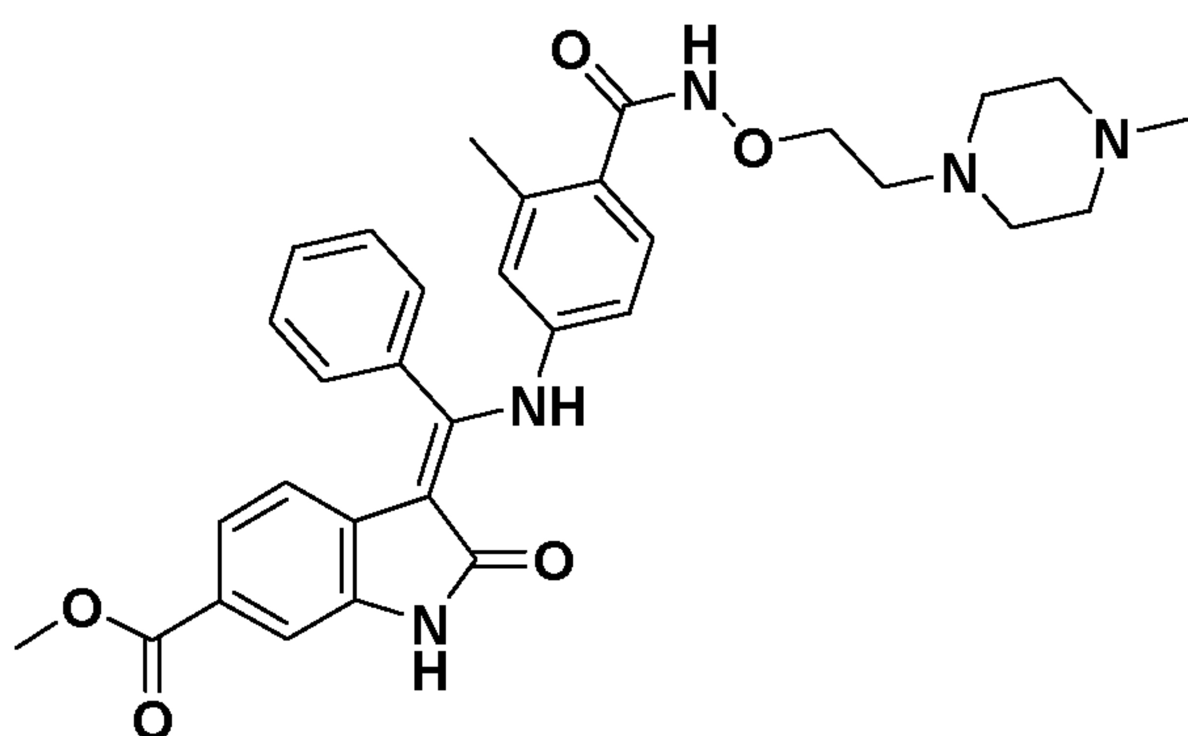
(Z)-Methyl 3-(((3-methyl-4-((2-(4-methylpiperazin-1-yl)ethoxy)carbamoyl)phenyl)amino)(phenyl)methylene)-2-oxoindoline-6-carboxylate
