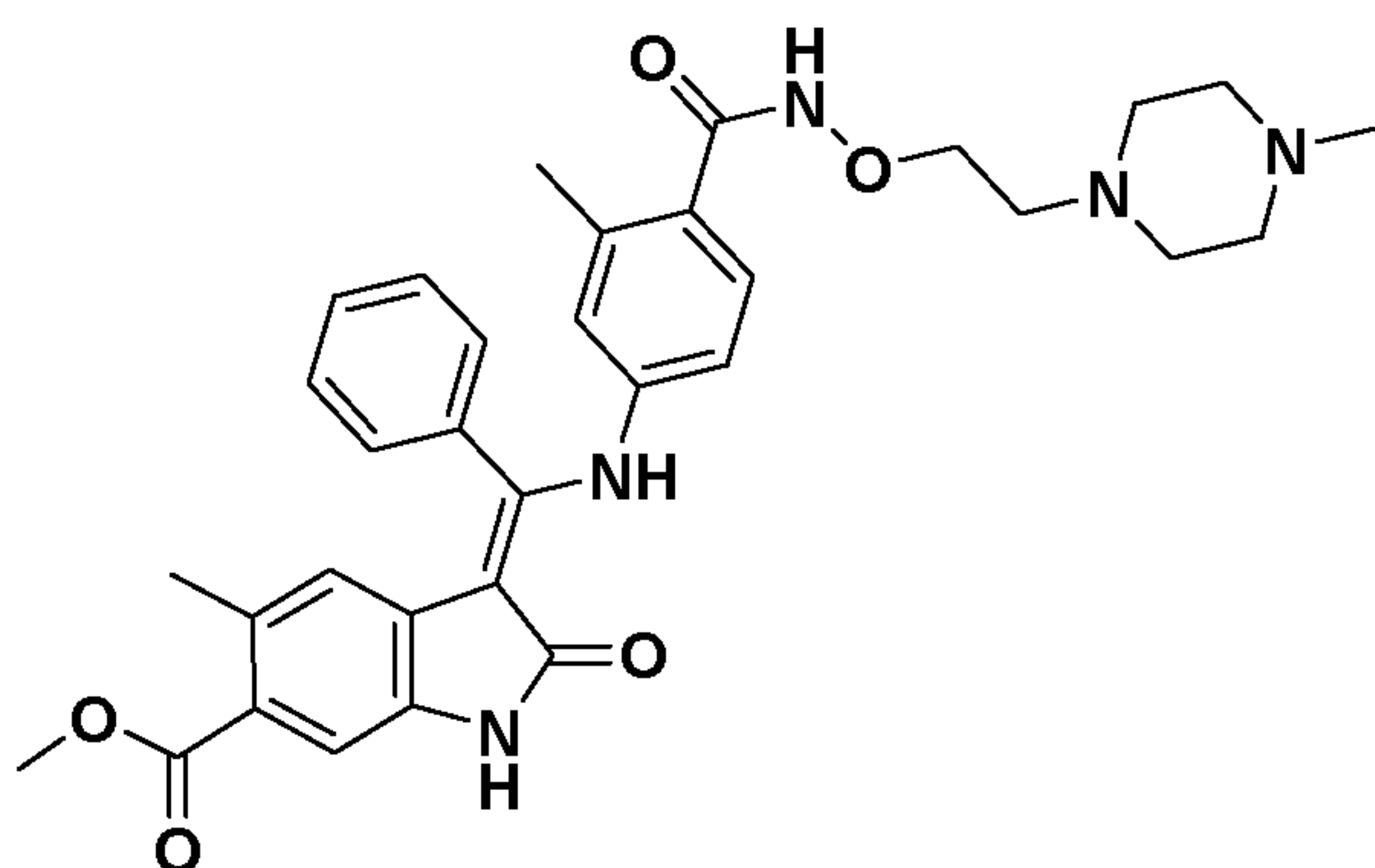
(Z)-Methyl 5-methyl-3-(((3-methyl-4-((2-(4-methylpiperazin-1-yl)ethoxy)carbonyl)phenyl)amino)(phenyl)methylene)-2-oxoindoline-6-carboxylate Route code*: 1B
