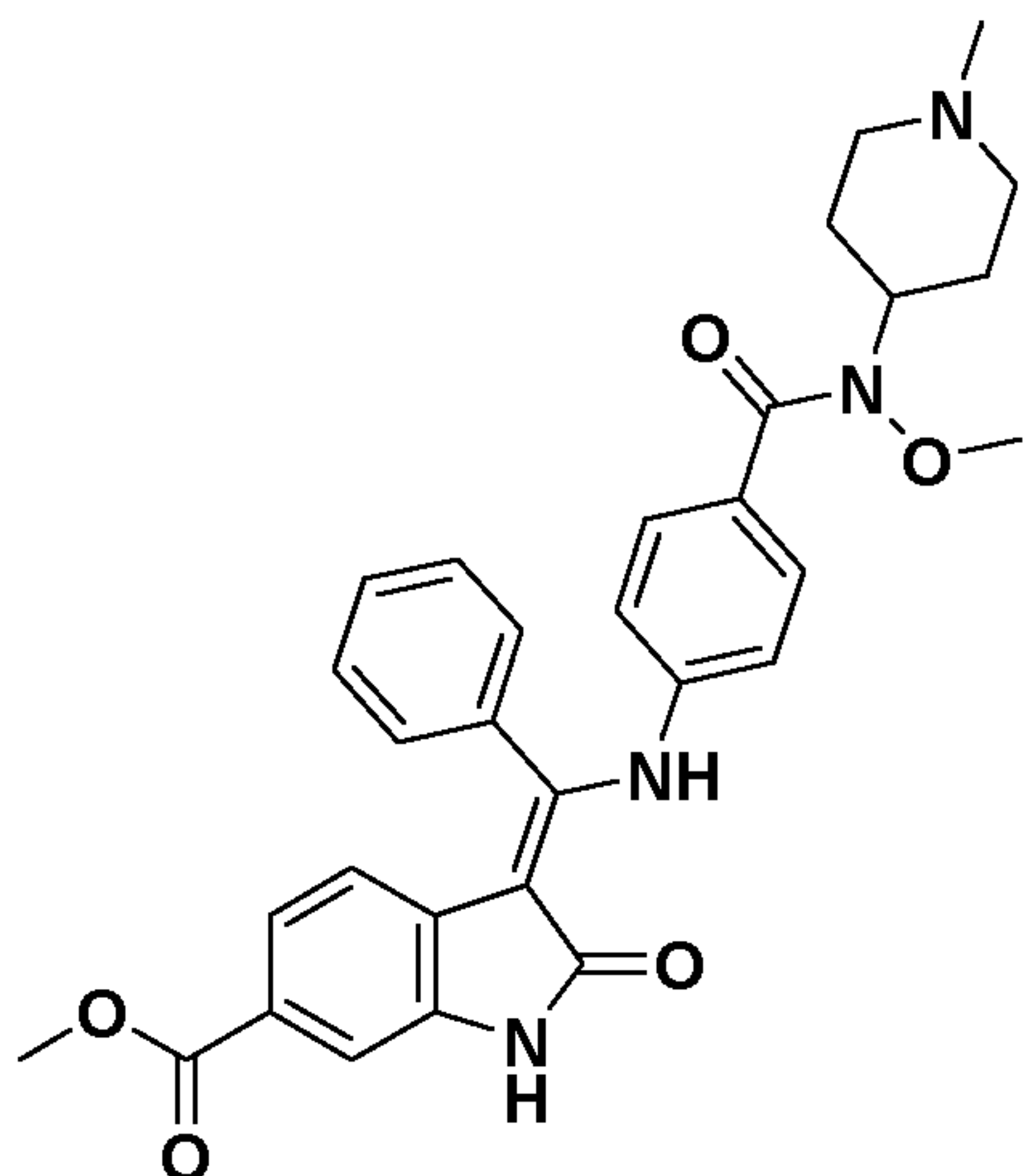
(Z)-Methyl 3-(((4-(methoxy(1-methylpiperidin-4-yl)carbamoyl)phenyl)amino)(phenyl)methylene)-2-oxoindoline-6-carboxylate
