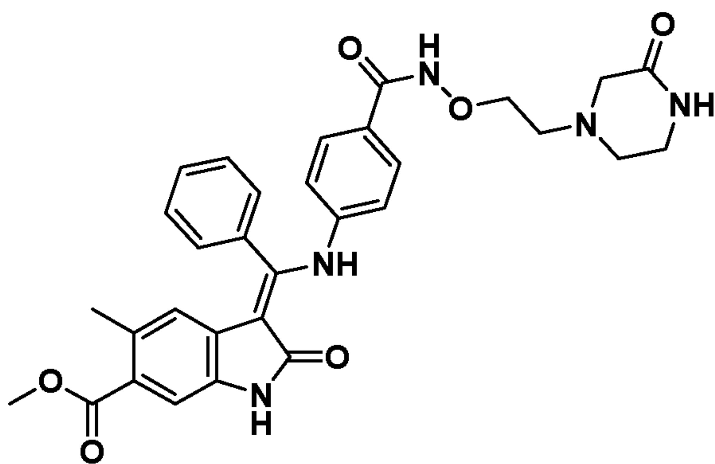
(Z)-Methyl 5-methyl-2-oxo-3-(((4-((2-(3-oxopiperazin-1-yl)ethoxy)carbamoyl)phenyl)amino)(phenyl)methylene)indoline-6-carboxylate
