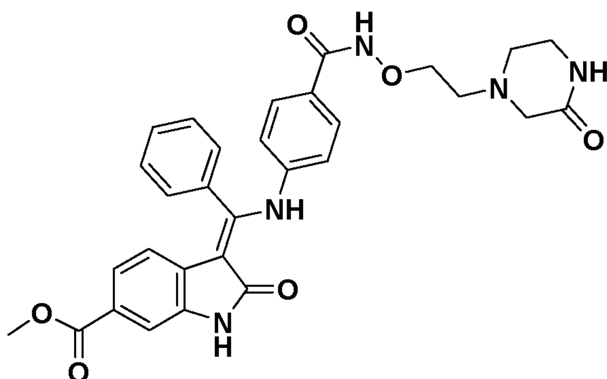
(Z)-Methyl 2-oxo-3-(((4-((2-(3-oxopiperazin-1-yl)ethoxy)carbamoyl)phenyl)amino)(phenyl)methylene)indoline-6-carboxylate Route code*: 1C
