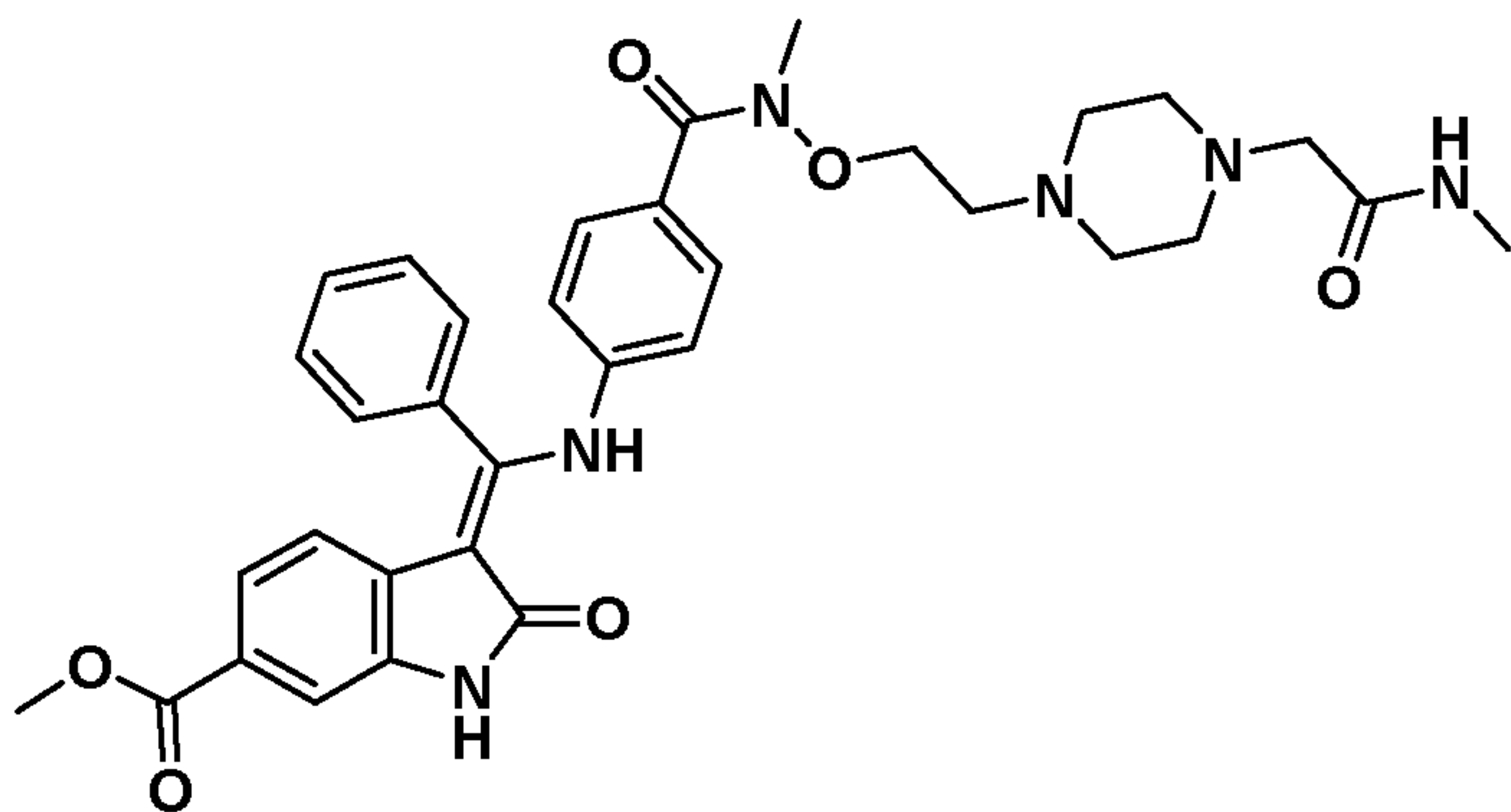
(Z)-Methyl 3-(((4-(methyl(2-(4-(2-(methylamino)-2-oxoethyl)piperazin-1-
