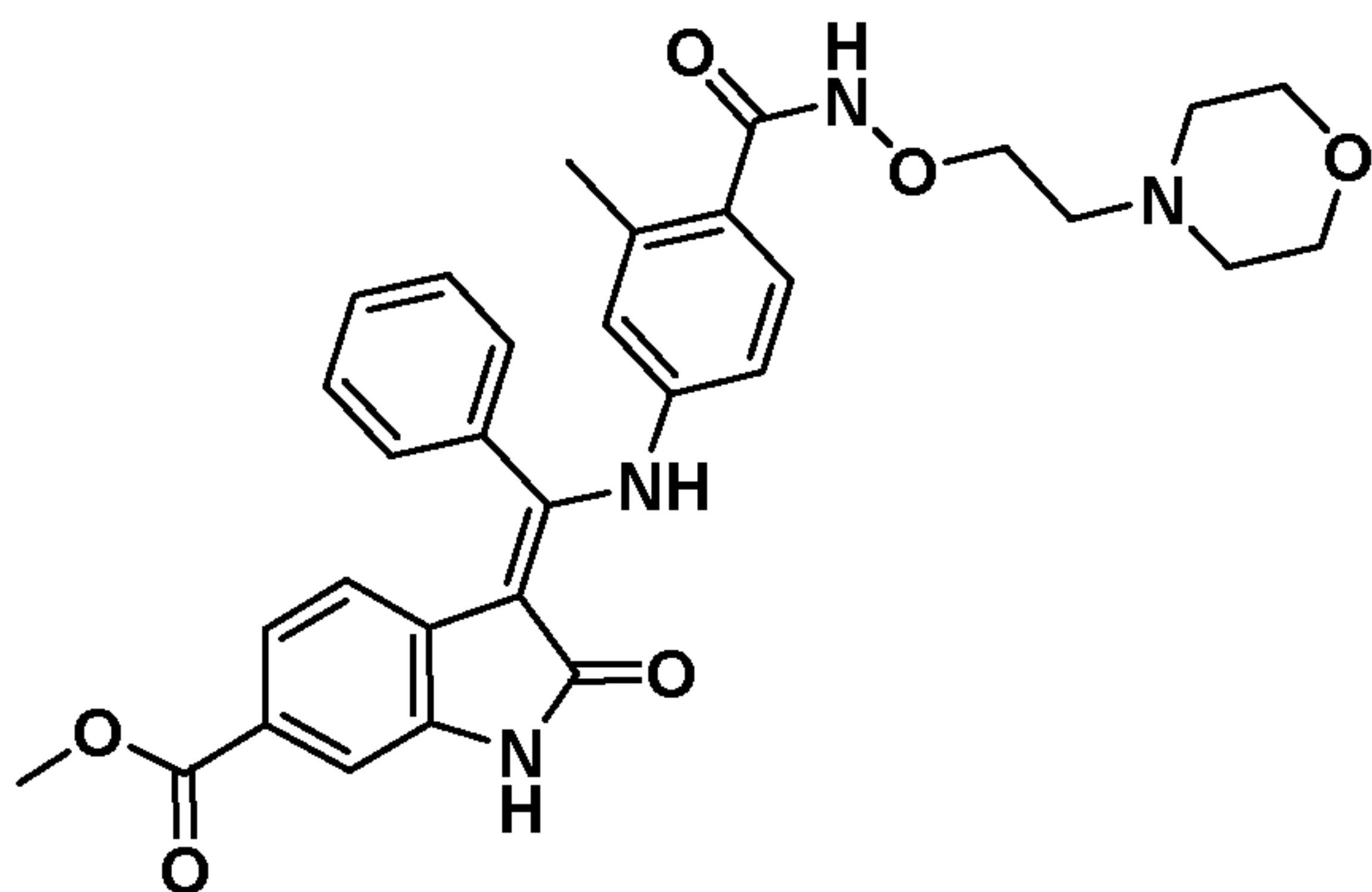
(Z)-Methyl 3-(((3-methyl-4-((2-morpholinoethoxy)carbamoyl)phenyl)amino)(phenyl)methylene)-2-oxoindoline-6-carboxylate
