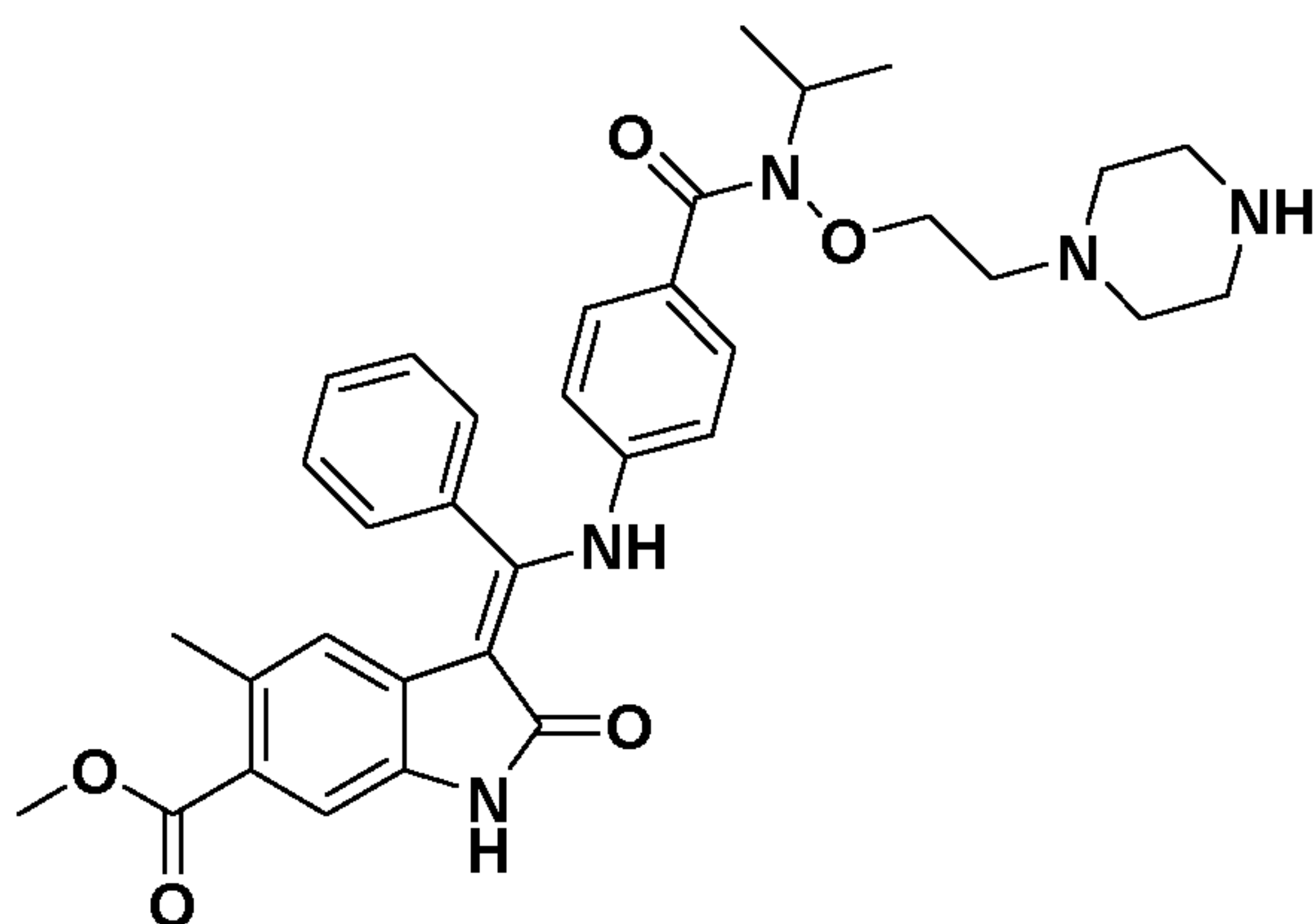
(Z)-Methyl 3-(((4-(isopropyl(2-(piperazin-1-yl)ethoxy)carbamoyl)phenyl)amino)(phenyl)methylene)-5-methyl-2-oxoindoline-6-carboxylate
