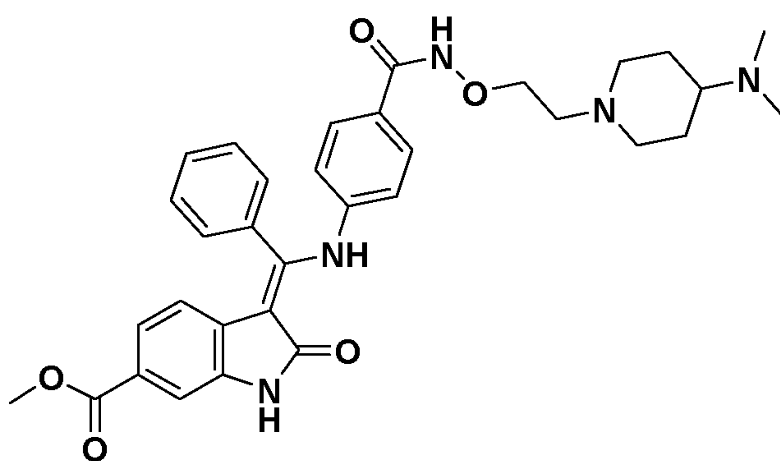
(Z)-Methyl 3-(((4-((2-(4-(dimethylamino)piperidin-1-yl)ethoxy)carbamoyl)phenyl)amino)(phenyl)methylene)-2-oxoindoline-6-carboxylate, formate
