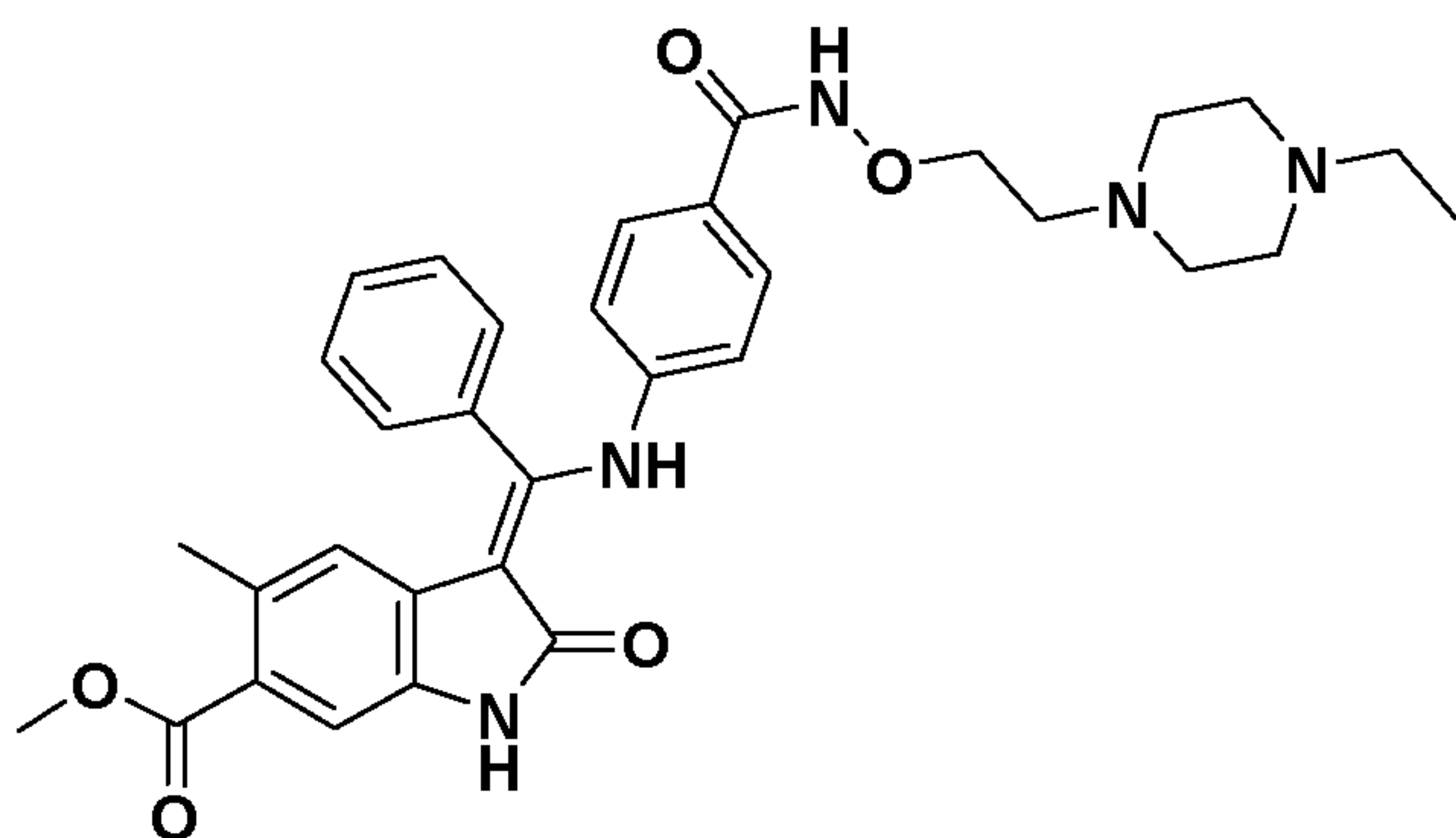
(Z)-Methyl 3-(((4-((2-(4-ethylpiperazin-1-yl)ethoxy)carbamoyl)phenyl)amino)(phenyl)methylene)-5-methyl-2-oxoindoline-6-carboxylate
