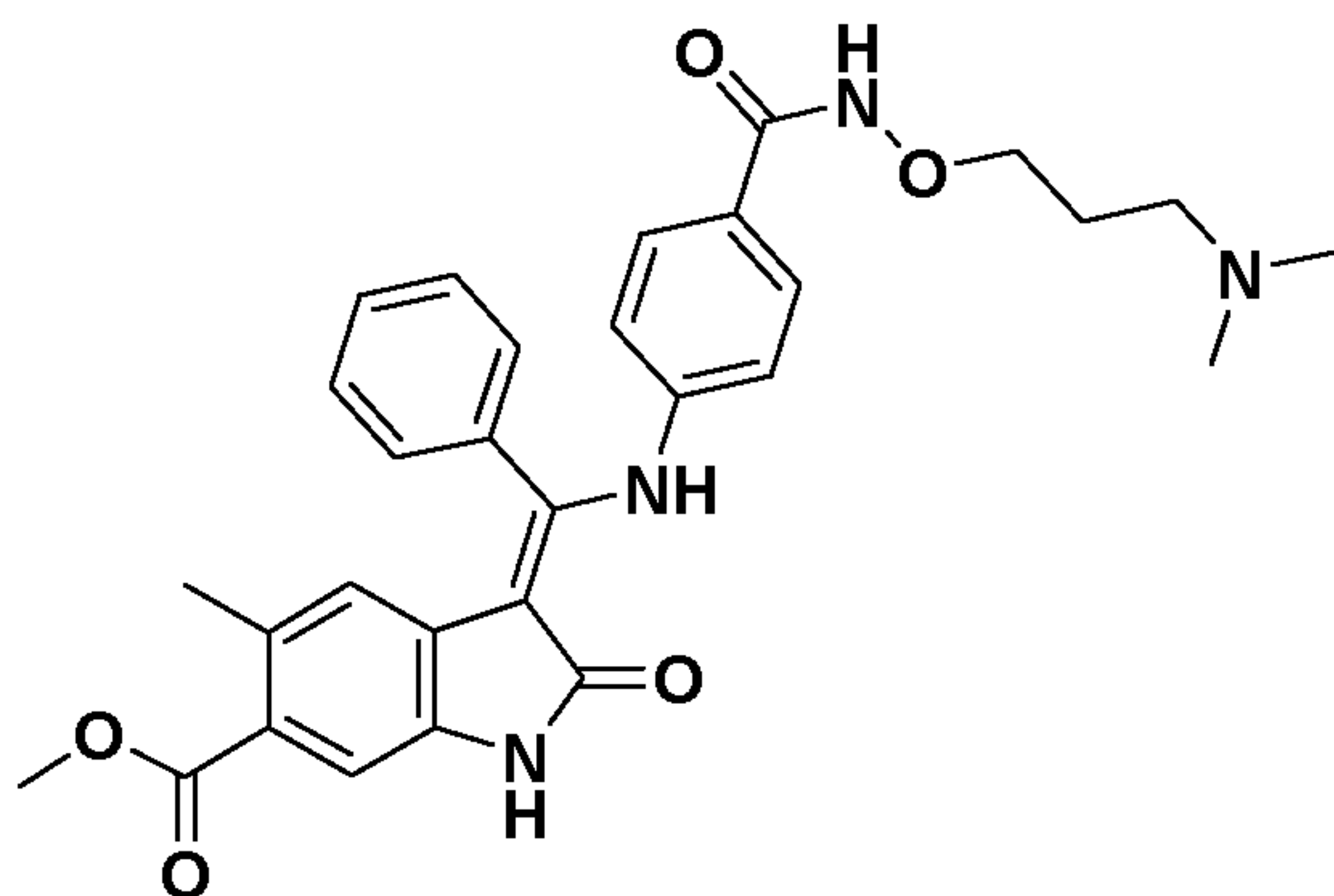
(Z)-Methyl 3-(((4-((3-(dimethylamino)propoxy)carbonyl)phenyl)amino)(phenyl)methylene)-5-methyl-2-oxoindoline-6-carboxylate Route code*: 1B
