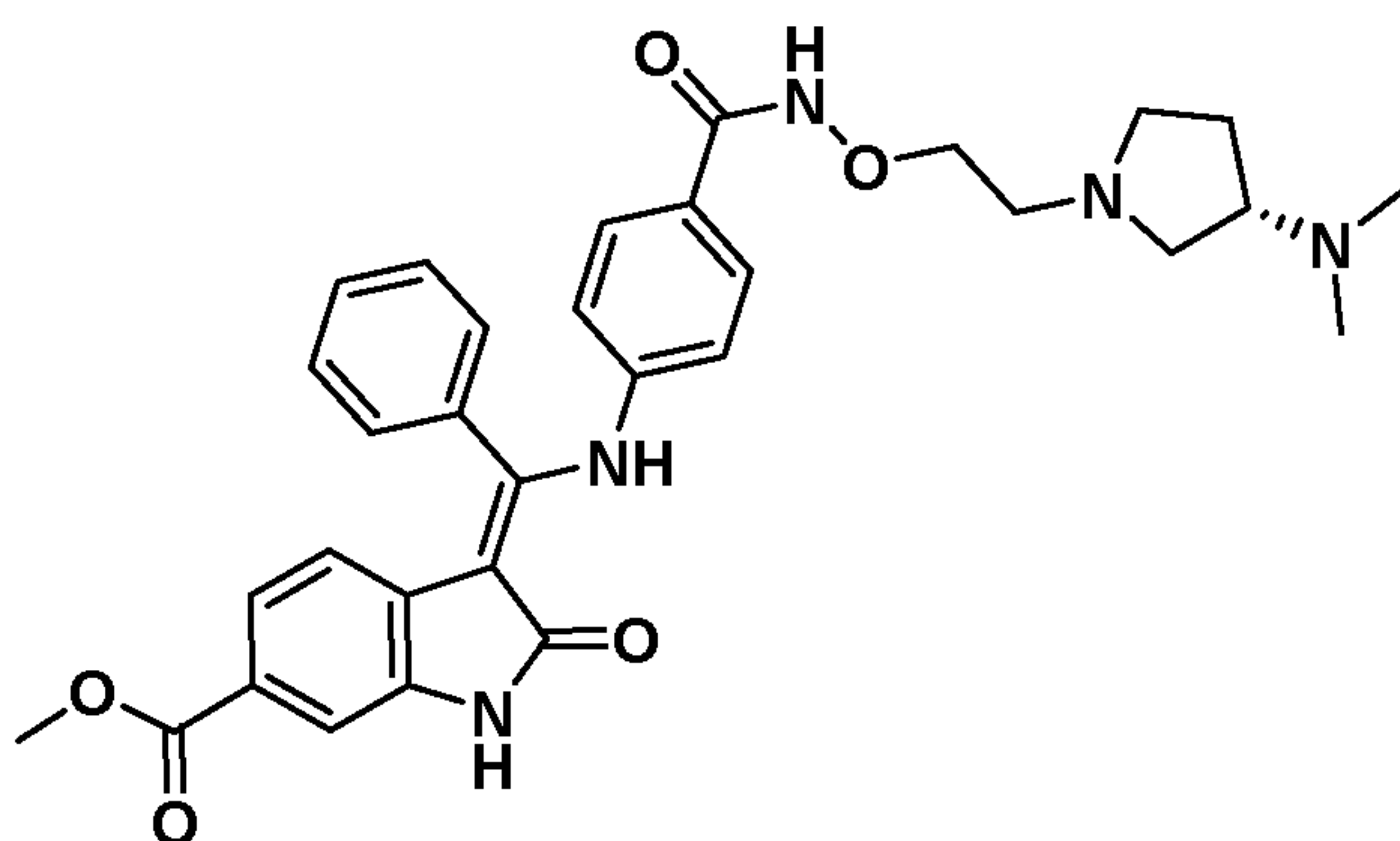
(S,Z)-Methyl 3-(((4-((2-(3-(dimethylamino)pyrrolidin-1-yl)ethoxy)carbamoyl)phenyl)amino)(phenyl)methylene)-2-oxoindoline-6-carboxylate, formate
