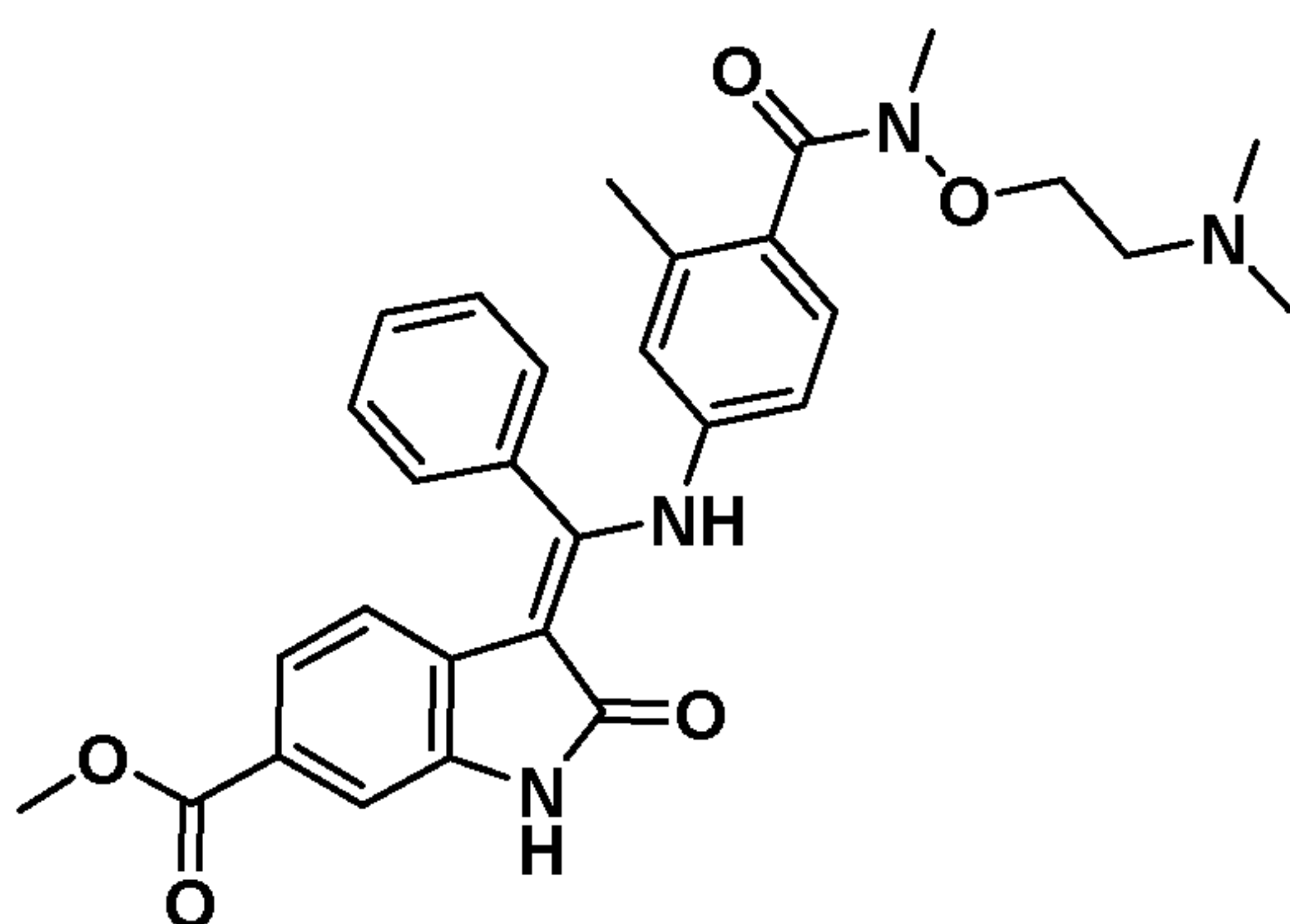
(Z)-Methyl 3-(((4-((2-(dimethylamino)ethoxy)(methyl)carbamoyl)-3-methylphenyl)amino)(phenyl)methylene)-2-oxoindoline-6-carboxylate
