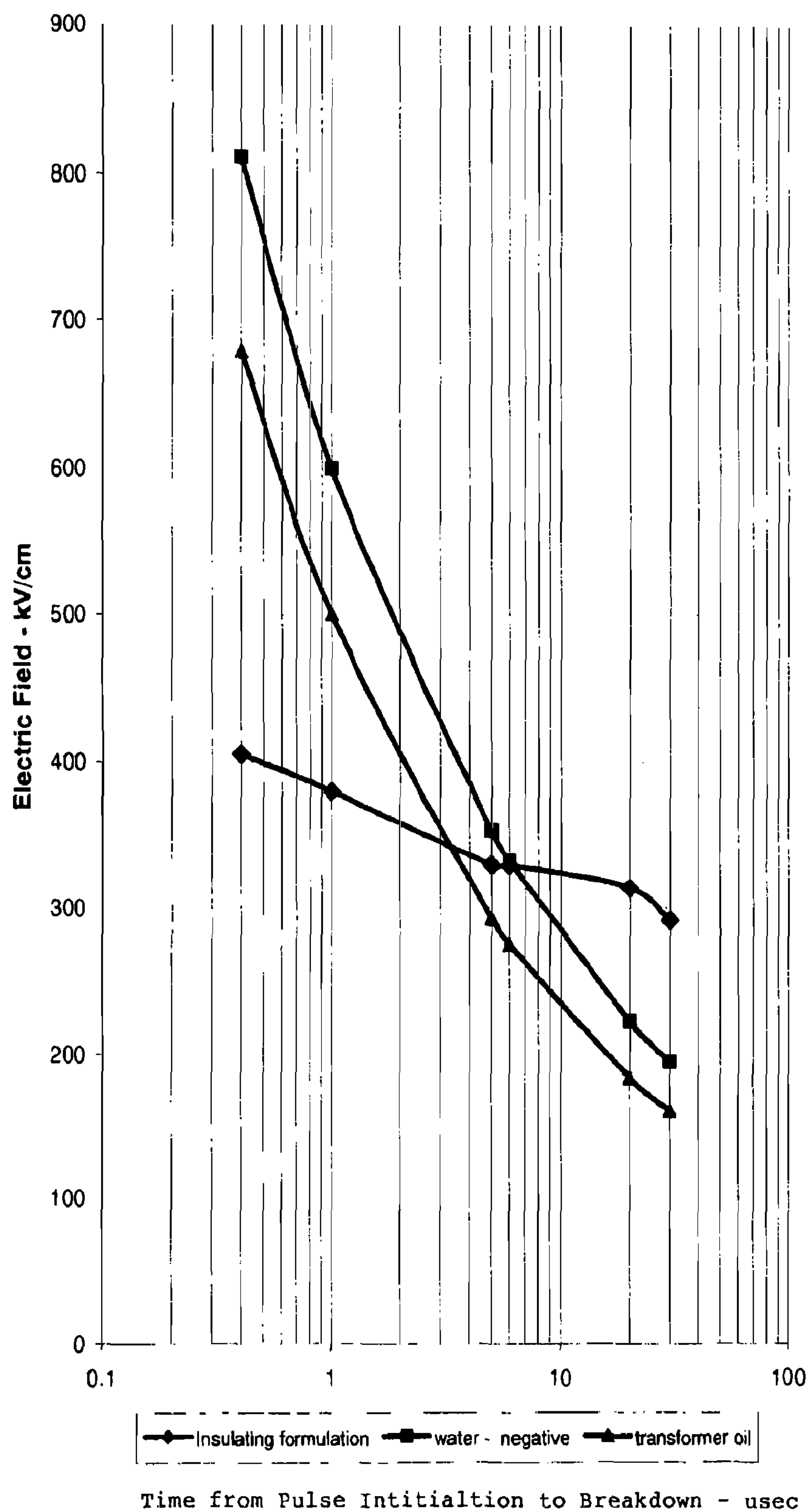
Dielectric Strength vs. Delay To Breakdown Figure 32
