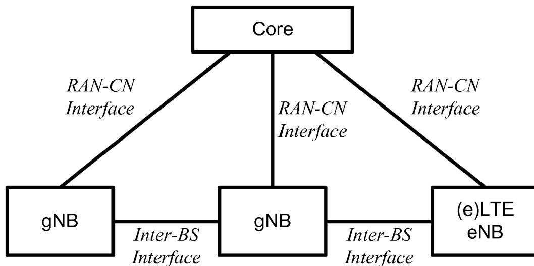
FIG. 13A Non-centralized deployment
