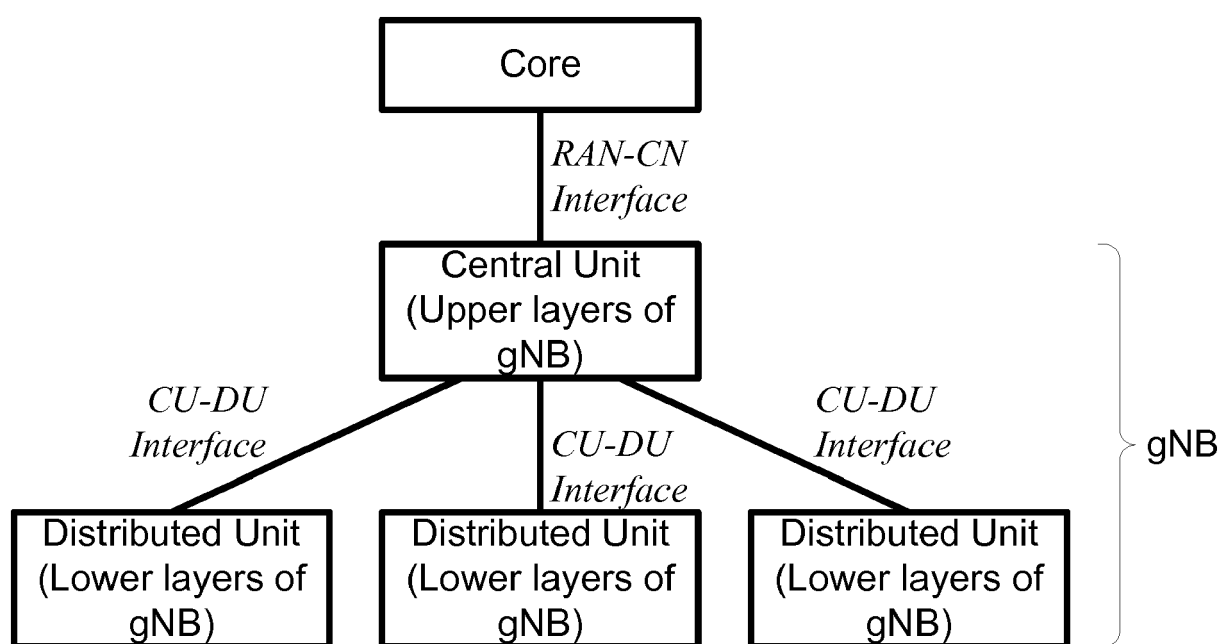
FIG. 13B Centralized deployment
