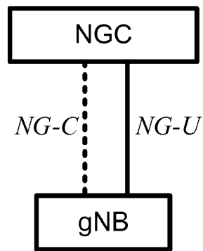
FIG. 10A gNB connected to NGC
