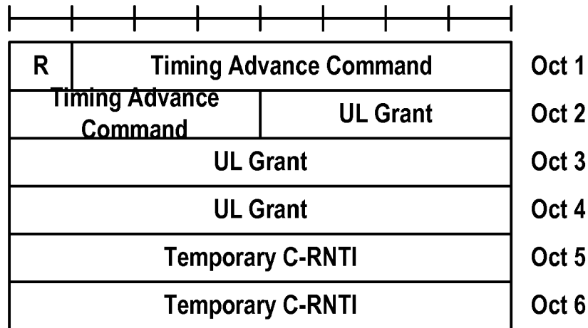
(A) MAC RAR
