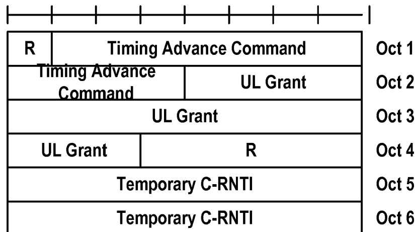
(C) MAC RAR for NB-IoT UEs
