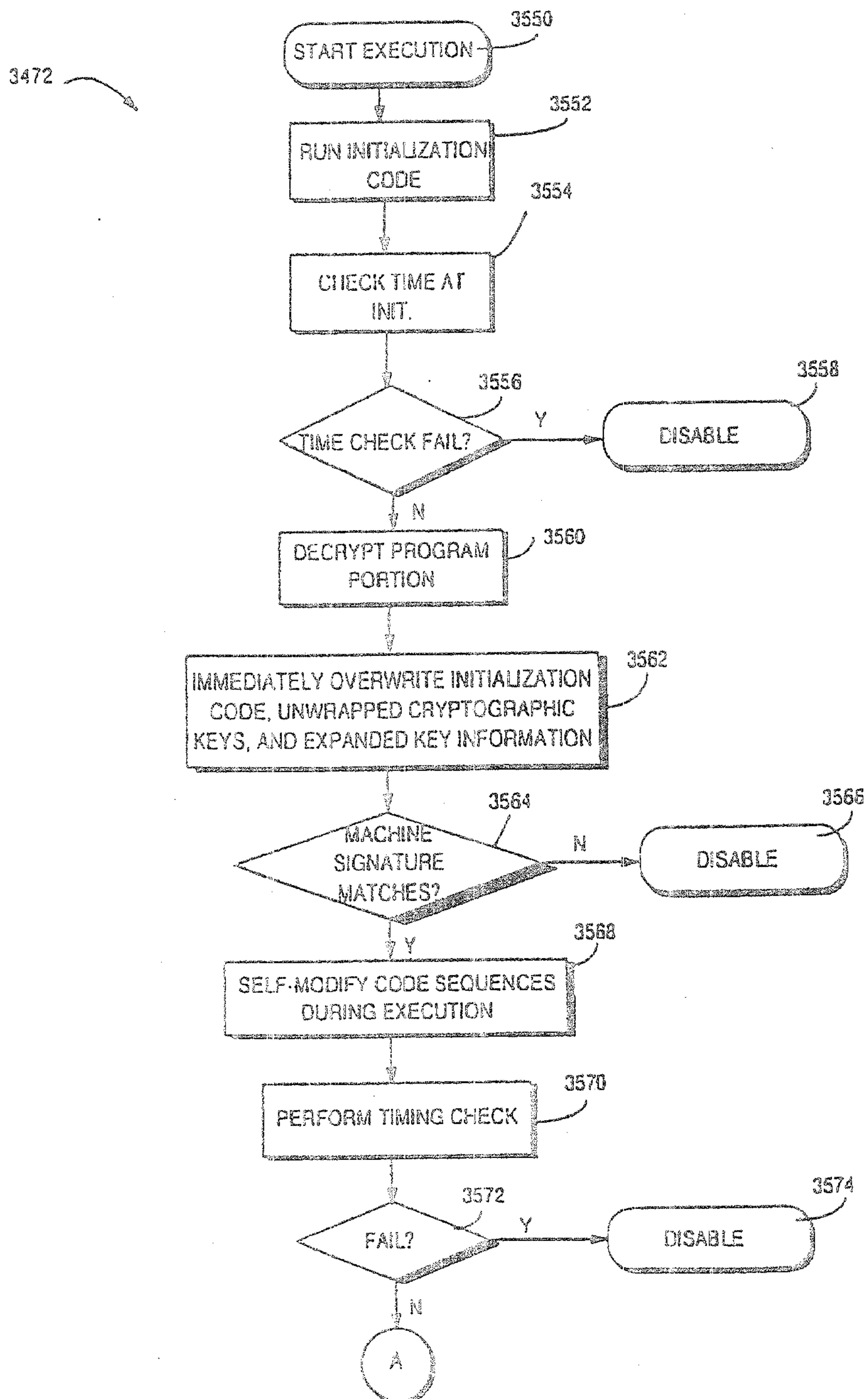
Fig. 69K Example Dynamic Protection Mechanisms
