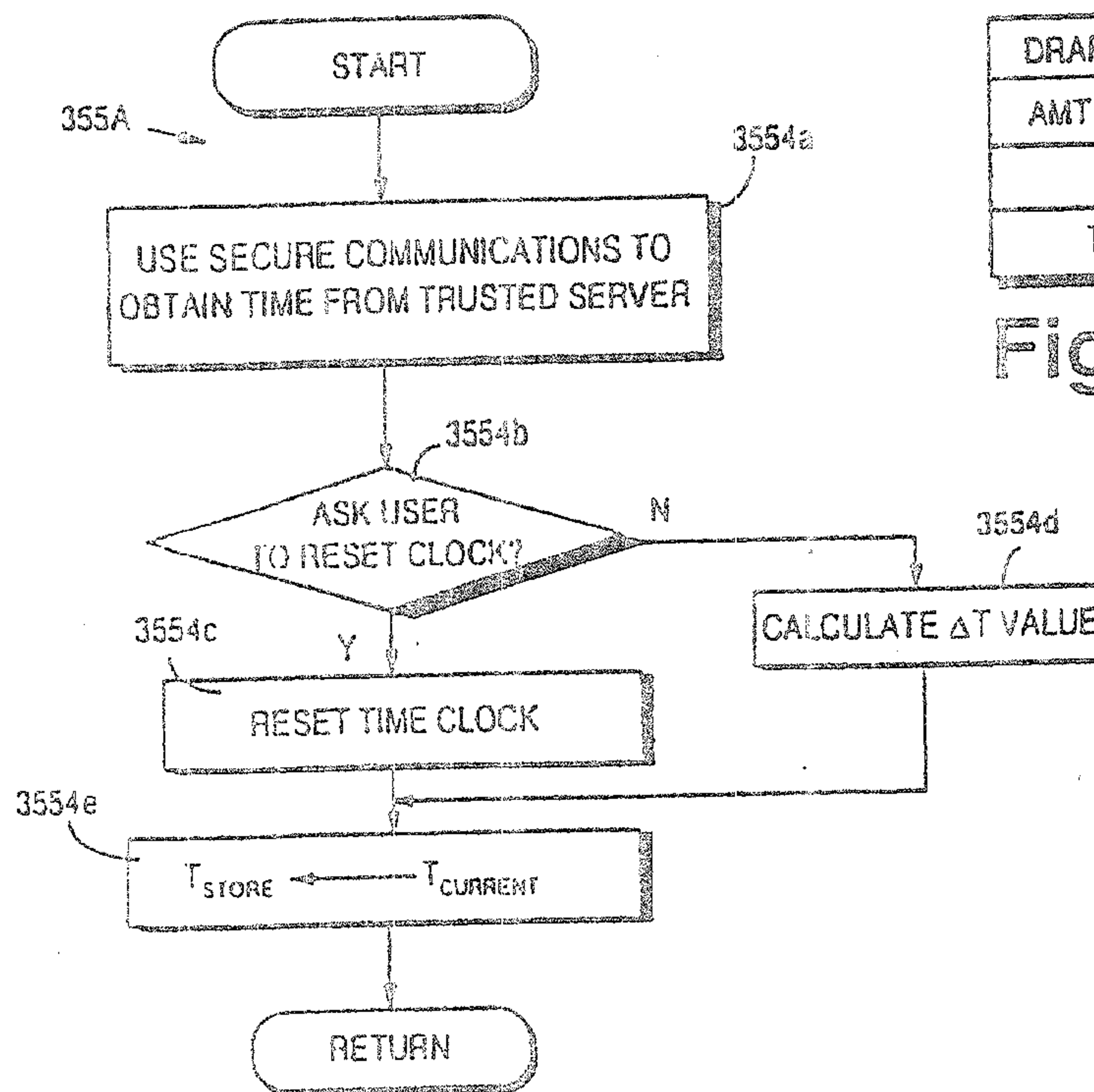
Fig. 69M Example Time Check At Initialization Routine
