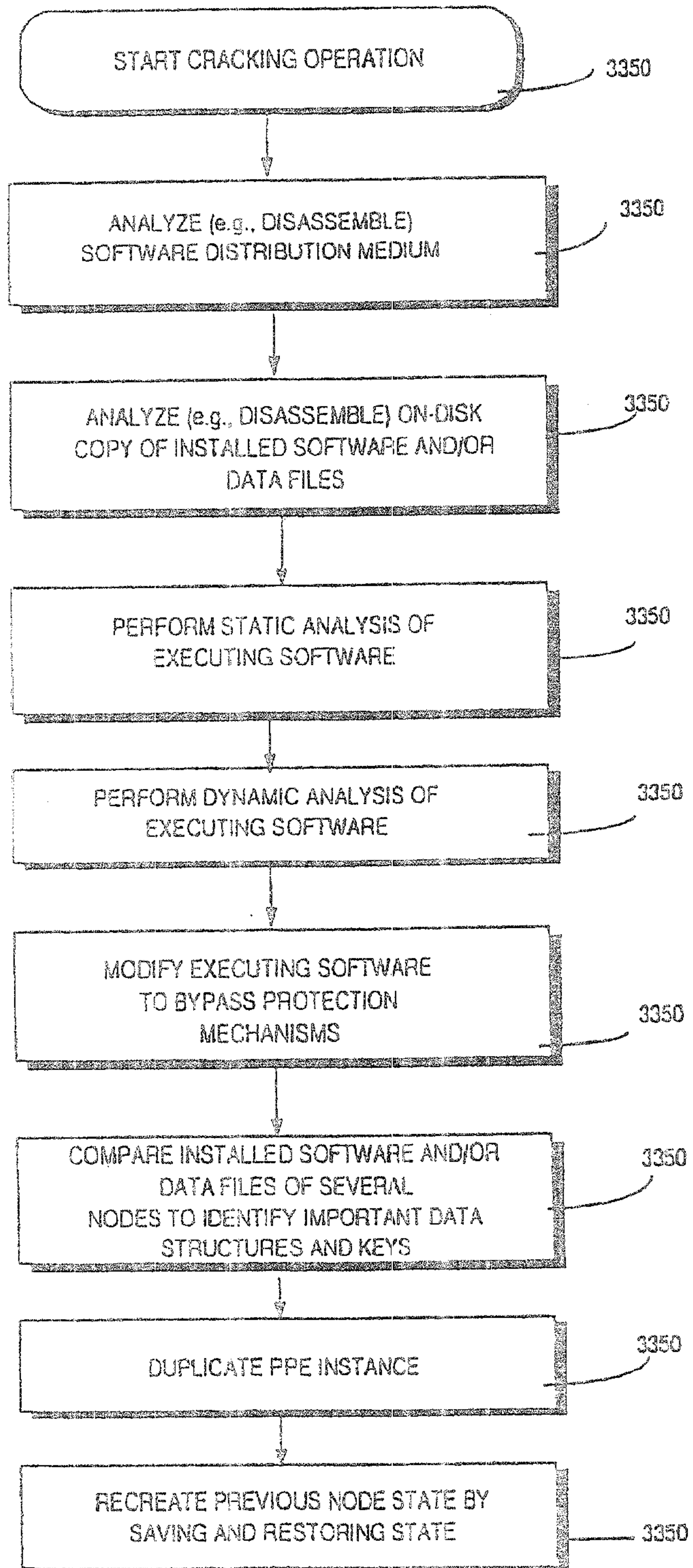
Fig. 67B Example Cracking Operation
