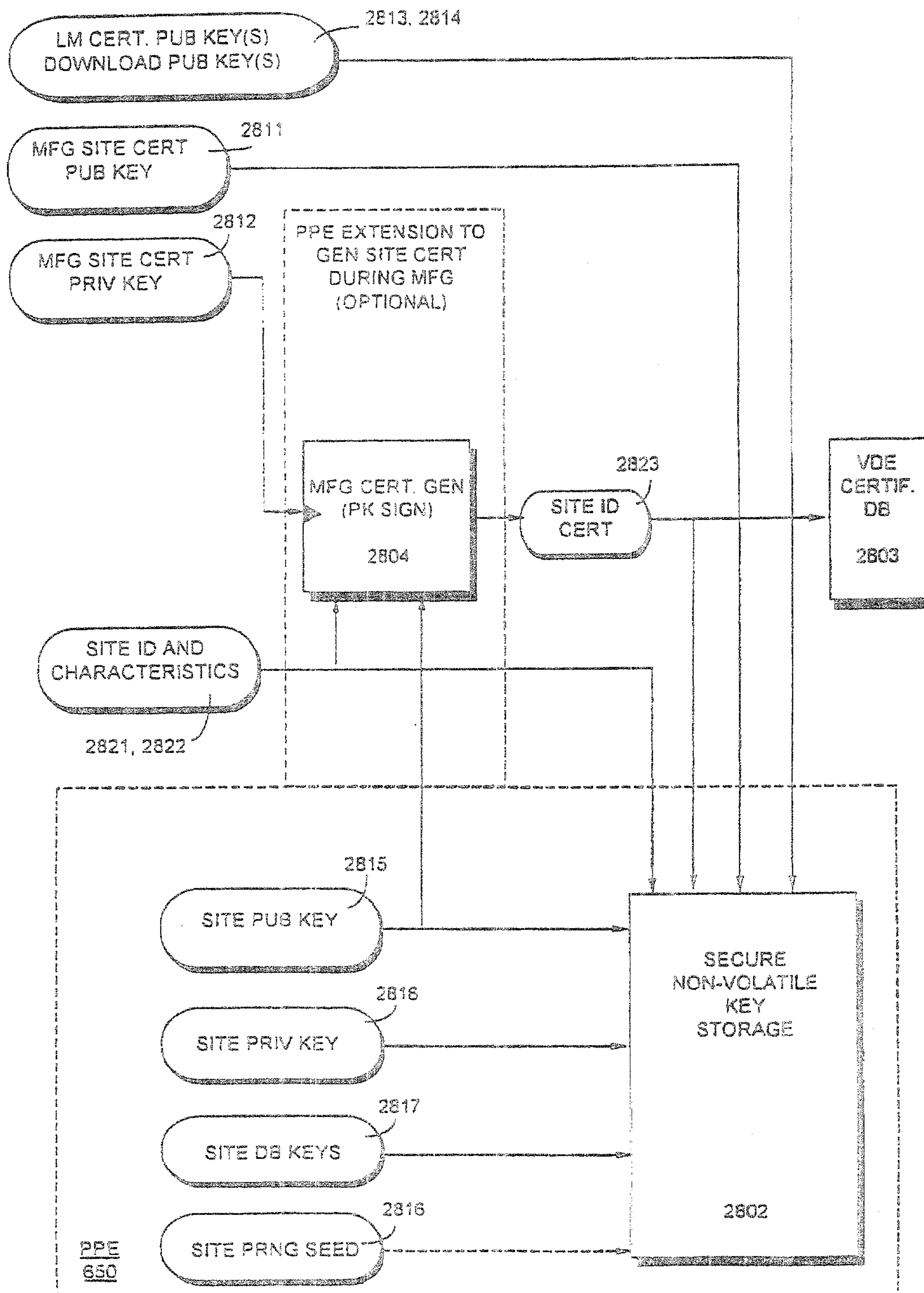
FIG. 64 SPU KEY INITIALIZATION/INSTALLATION
