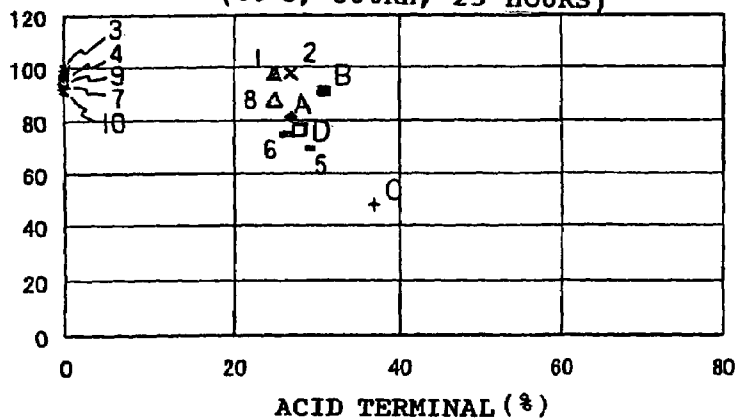
FIG. 4 RESULTS OF HYDROLYSIS TEST (60°C, 80%RH, 25 HOURS)
