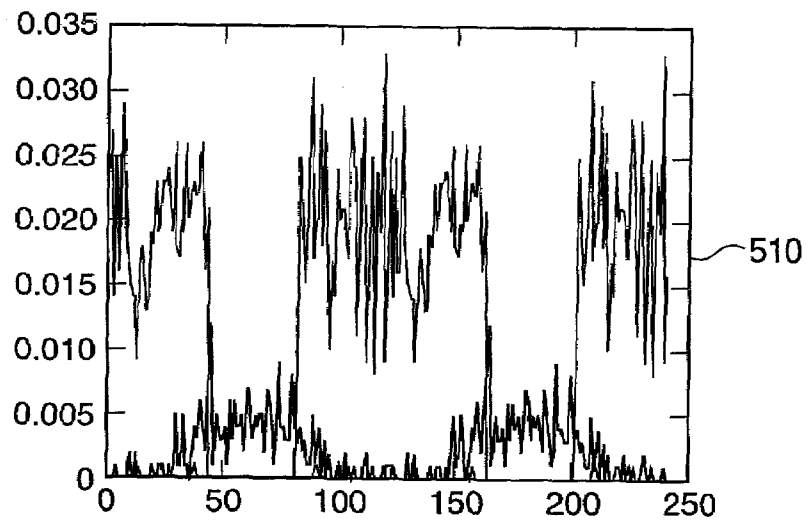
FIG. 5a 1.0 Torr
