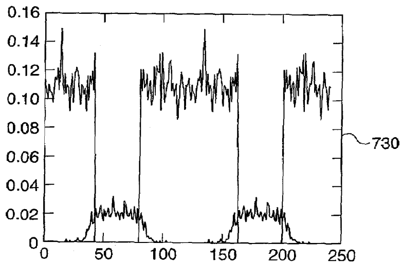
FIG. 7c t = 54 \mu\text{m}
