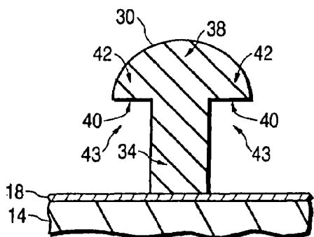
FIG. 3 (PRIOR ART)
