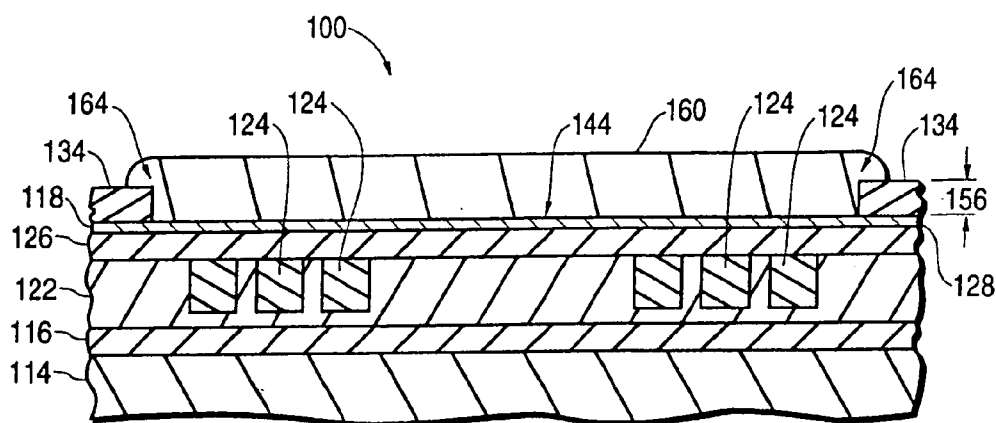
FIG. 18 (PRIOR ART)
