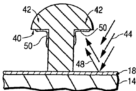
FIG. 4 (PRIOR ART)
