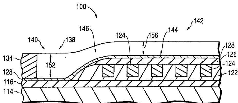
FIG. 16 (PRIOR ART)
