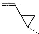
Vinylcyclopropyl
