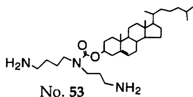
N^4 -spermidine cholesteryl carbamate
