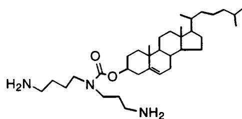
( spermidine cholesterol carbamate )
