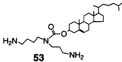
53 N 4 -spermidine cholesteryl carbamate
