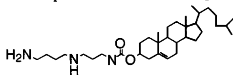
(N 1 -spermidine cholesteryl
