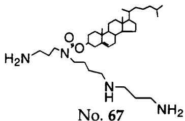
N^4 -spermine cholesteryl carbamate
