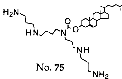
5 N^1,N^8 -Bis (3-aminopropyl)- N^4 -spermidine cholesteryl carbamate
