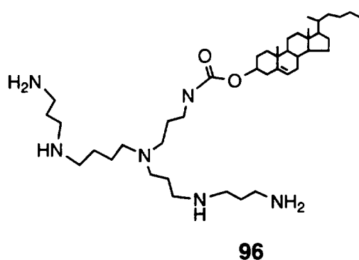
N-[N 1 ,N 4 ,N 8 -Tris(3-aminopropyl) spermidine] cholesteryl carbamate
