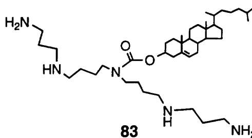
N,N-Bis(N'-3-aminopropyl-N''-4-aminobutyl) cholesteryl carbamate
