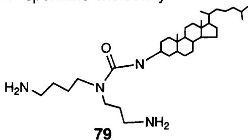
N 4 -spermidine dihydro cholesteryl urea
