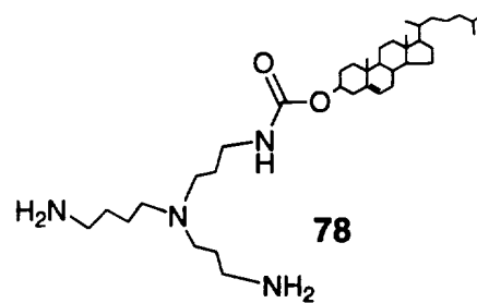
78 N(N 4 -3-aminopropyl)spermidine cholesteryl carbamate
