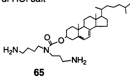
65 N 4 -spermidine-7 dehydro cholesteryl carbamate
