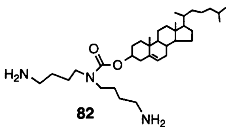
N,N-Bis(4-aminobutyl) cholesteryl carbamate
