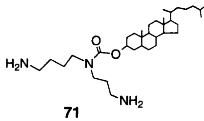
71 N 4 -spermidine dihydrocholesteryl carbamate
