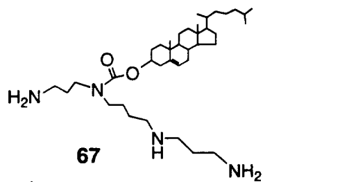
67 N 4 -spermine cholesteryl carbamate
