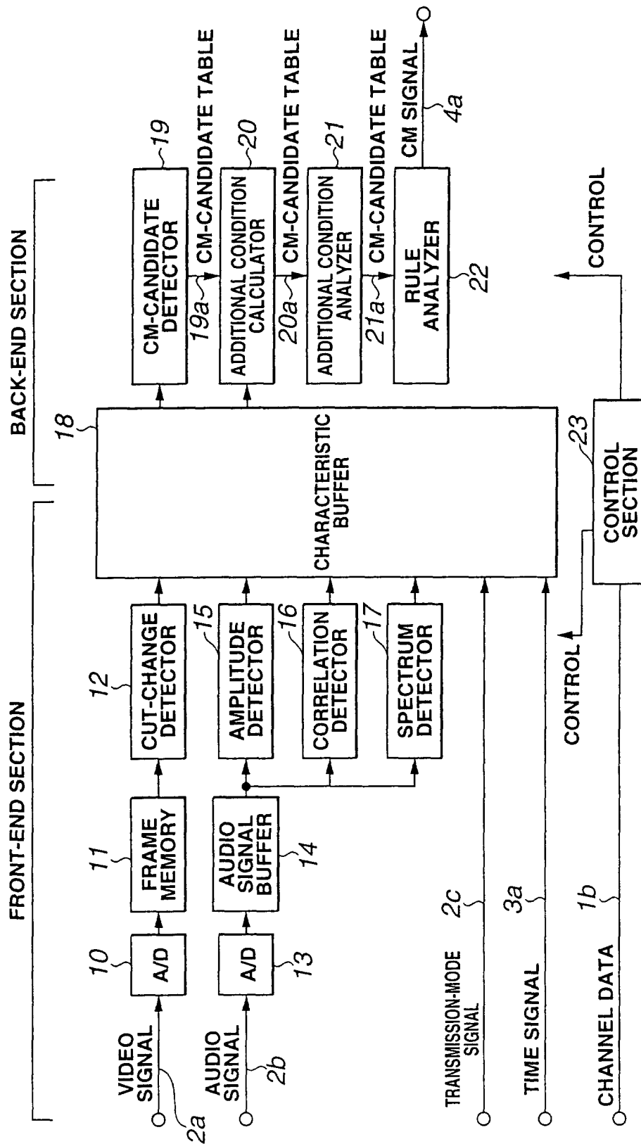
CM-DETECTING SECTION 4
