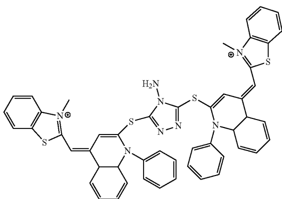
Example 33
