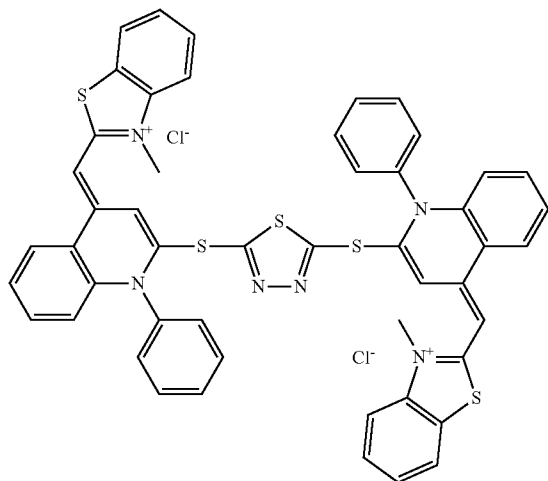
Compound 7
