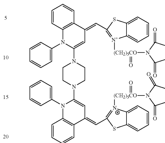
Compound 32
