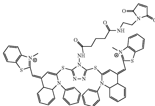
Example 35
