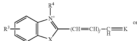
Formula (III)(y)
