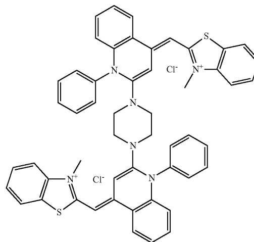
Compound 6
