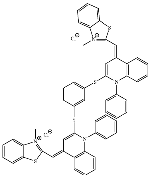
Example 25
