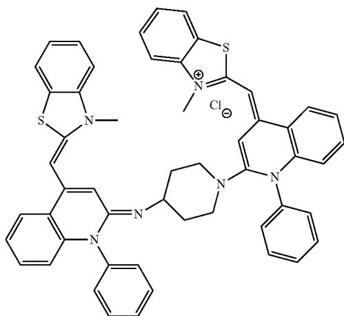
Compound 30
