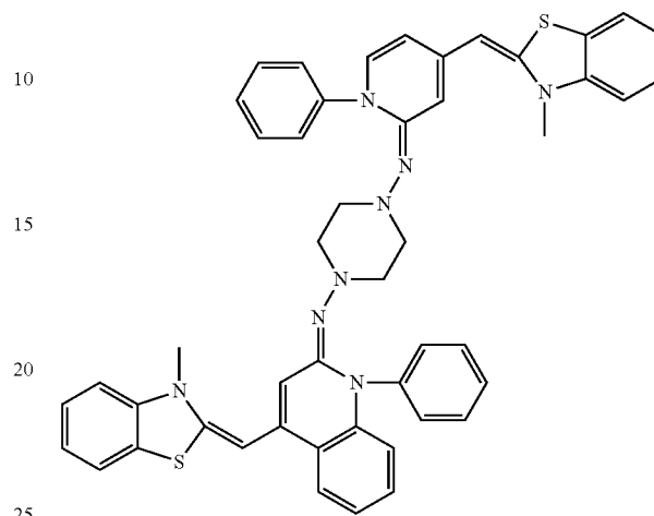
Example 26
