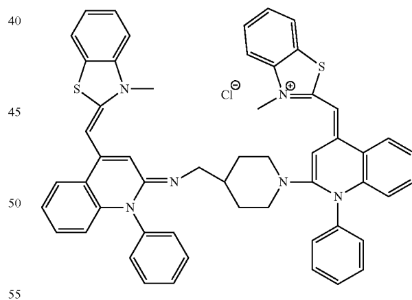
Example 27
