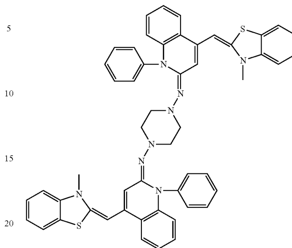
Compound 9
