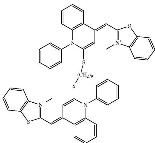
Compound 1
