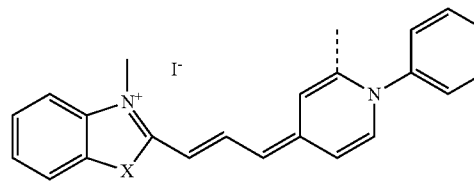
Formula (III)(c)
