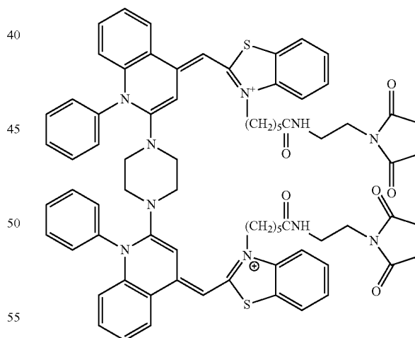
Compound 33
