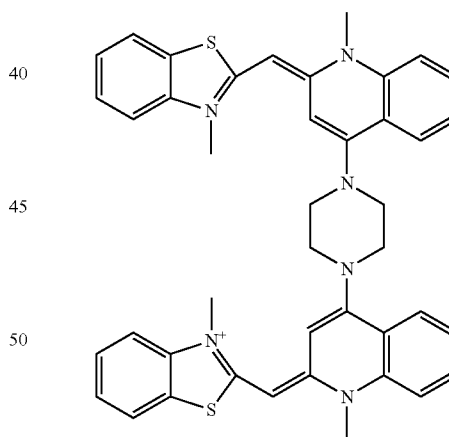
Example 11
