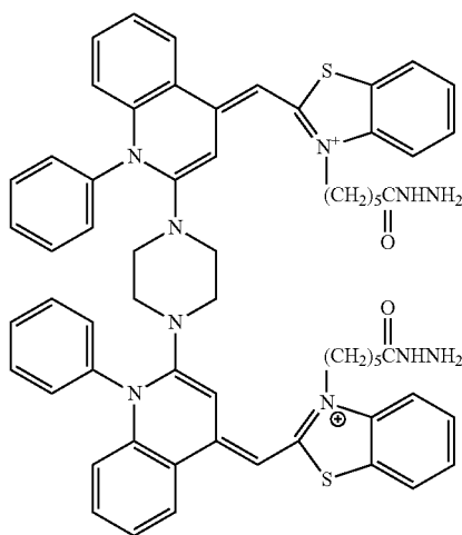
Example 32
