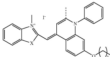
Formula (III)(e)
