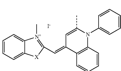
Formula (III)(a)
