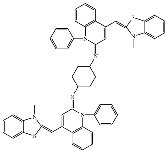
Compound 8
