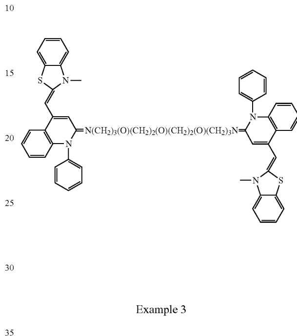
Compound 1
