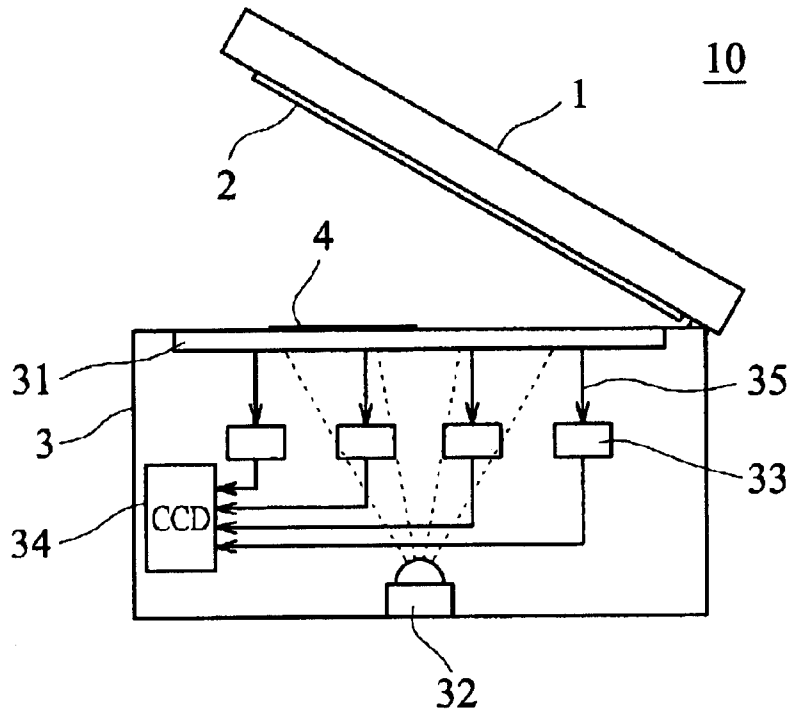
FIG. 1 (PRIOR ART)
