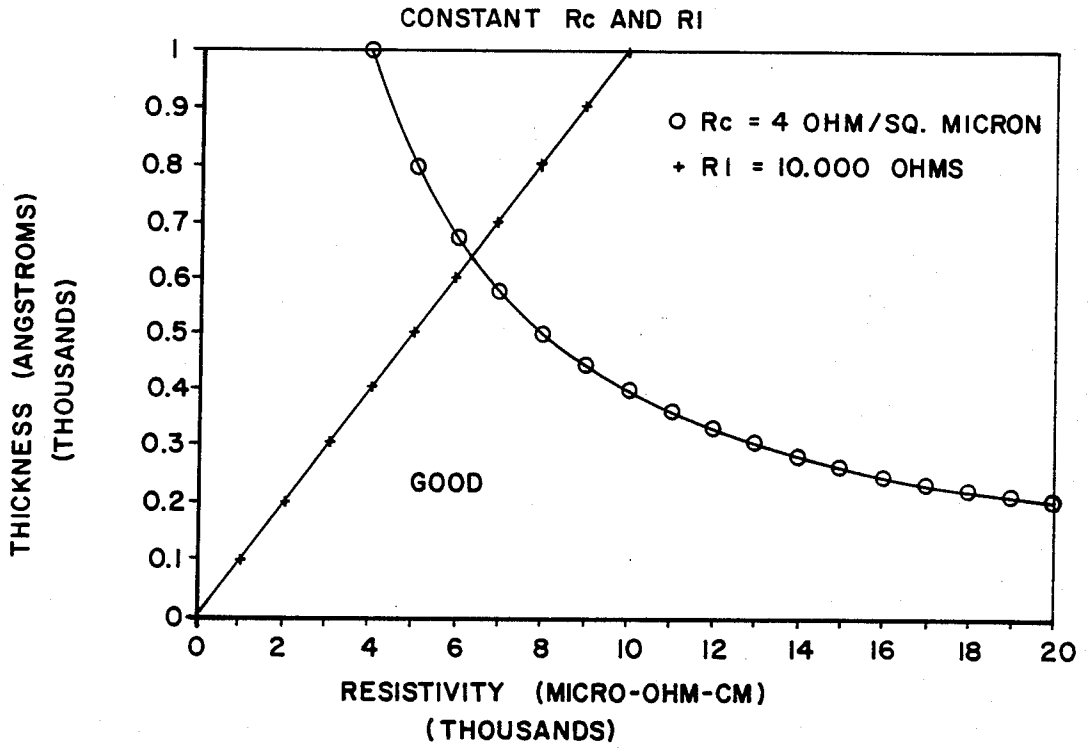
Fig. 5 (RESISTIVE LAYER)
