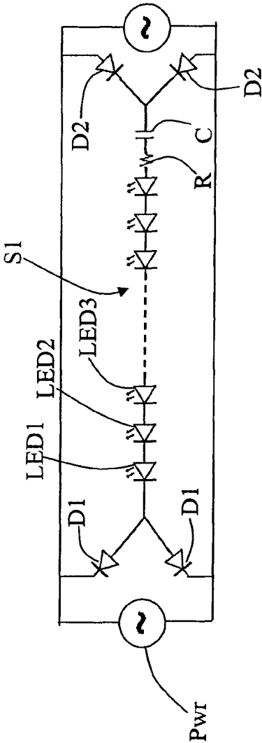
FIG. 3 (Prior Art)
