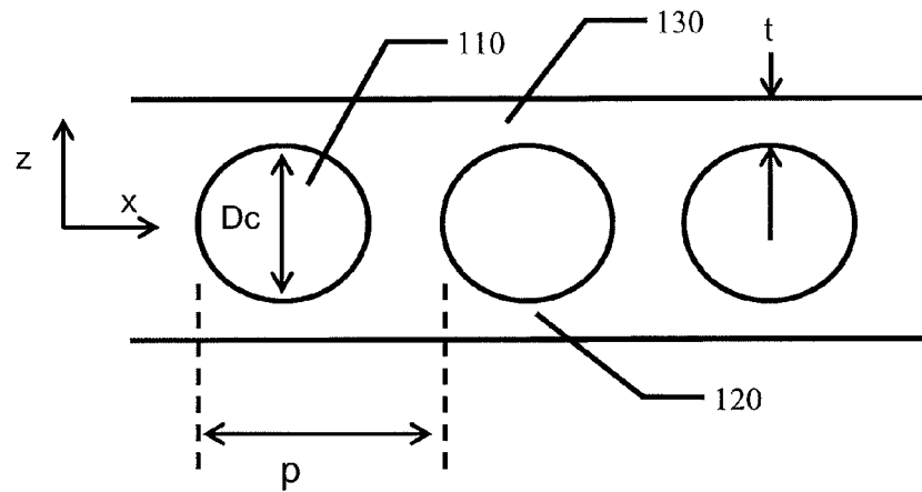
Fig. 16 – Simple example for beam web geometry
