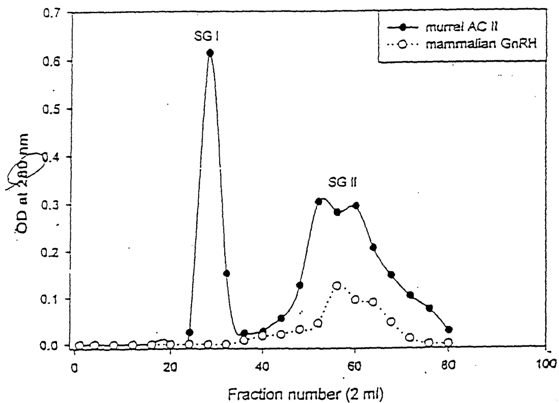
Fig 4. Elution profile of mammalian GnRH through Sephadex G-25 column. AC II fraction was dissolved in 1N acetic acid and eluted through Sephadex G-25 column (58x1.5 cm) at a flow rate of 24 ml/hr.
