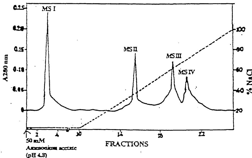
Fig. 5'b. Elution profile of murrel Mono Q unbound peak (MQ I) through FPLC Mono S column.
