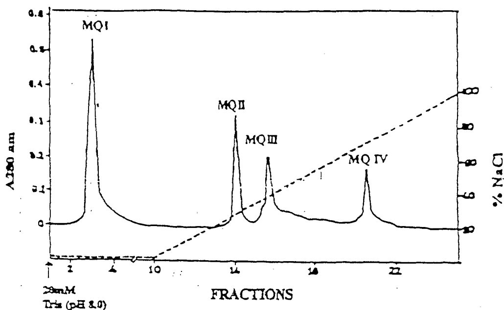
Fig. 5'a. Elution profile of murrel Sephadex G-25 P-II through FPLC Mono Q column.
