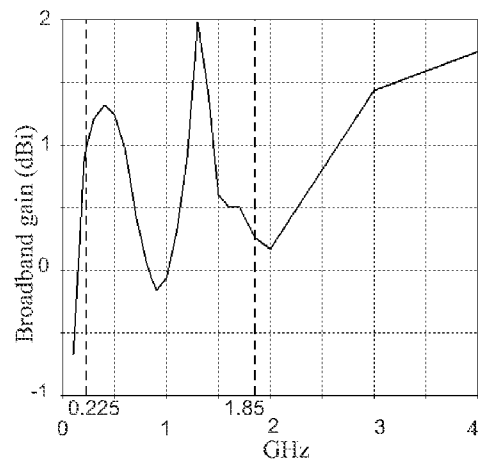
Gain at Elevation = 0 deg.; Azimuth = 90 deg.
