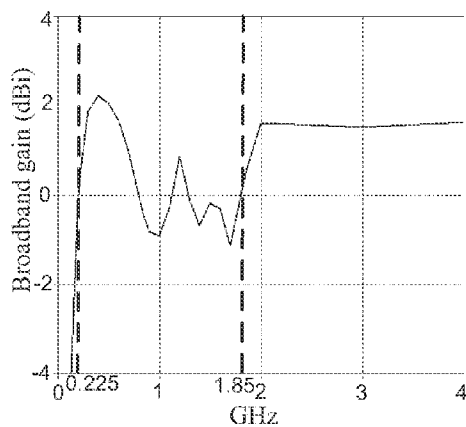
Gain at Elevation = 0 deg.; Azimuth = 90 deg.
