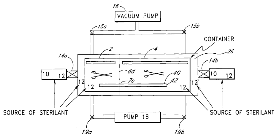
THE USE OF CONTAINER IN THE SYSTEM— CONFIGURATION 3
