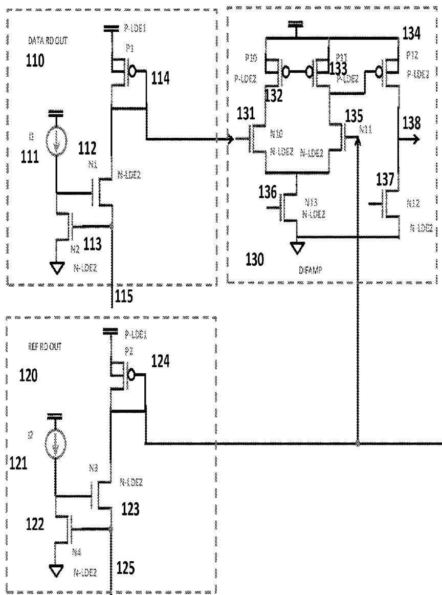
FIGURE 2 Sensing Circuit 100
