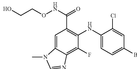
Compound 1
