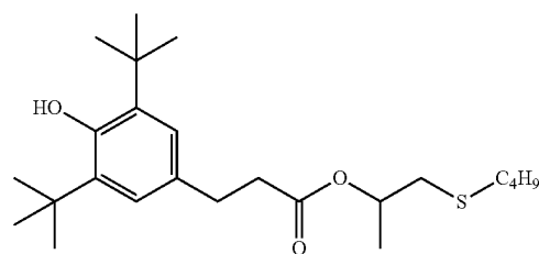
Formula (II) 10
