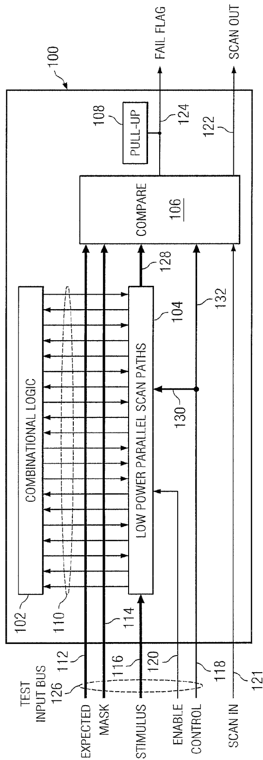
FIG. 1 (PRIOR ART)
