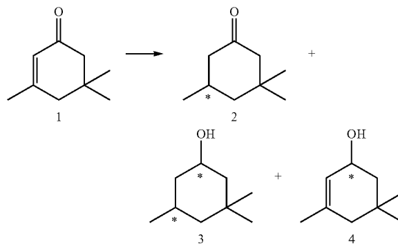
Scheme A: Asymmetric hydrogenation of isophorone 1
