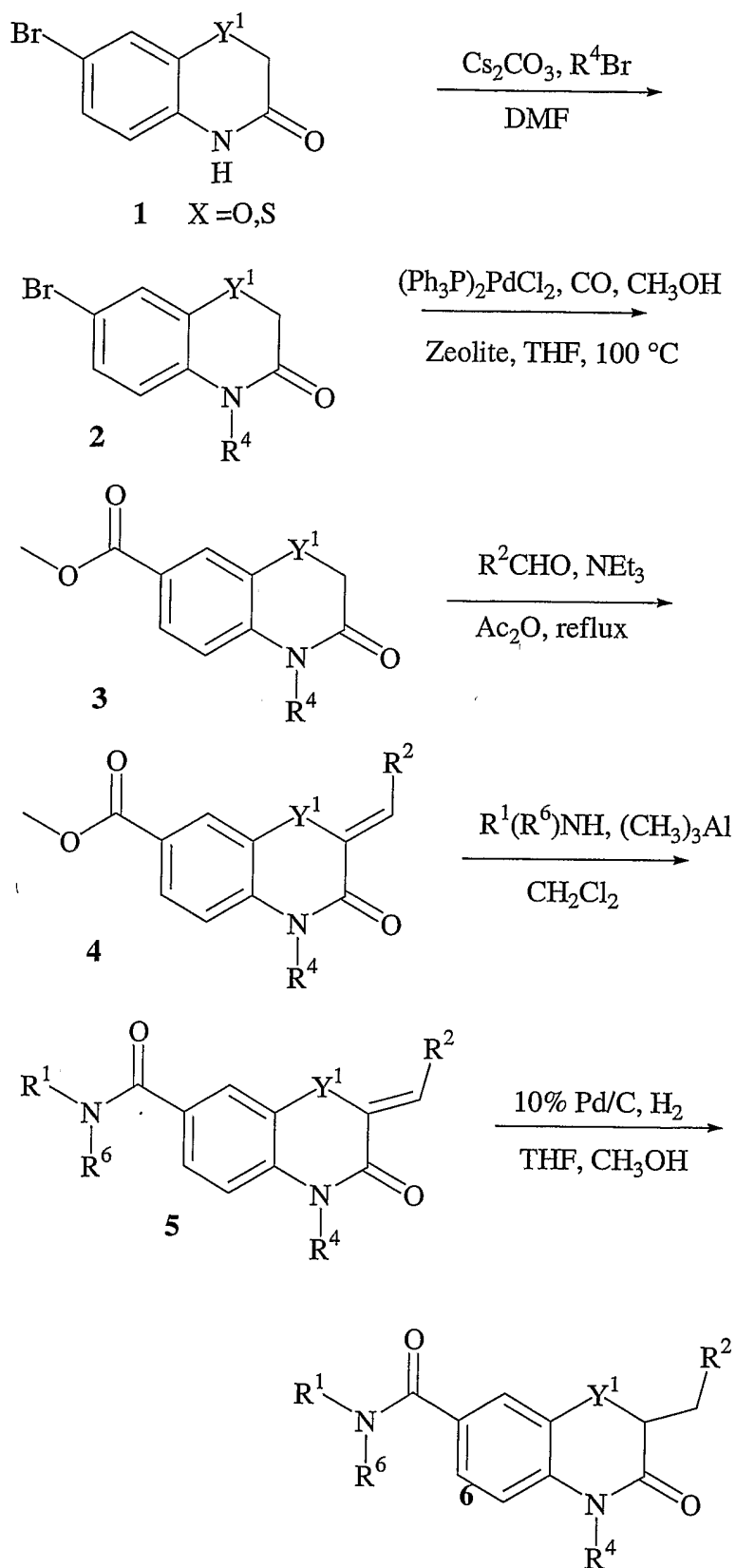
Scheme 1.
