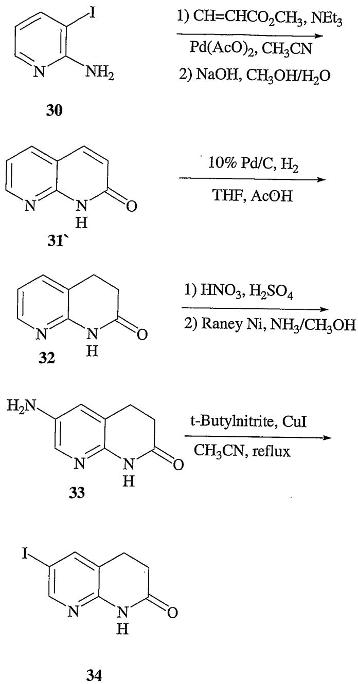
Scheme 4b.
