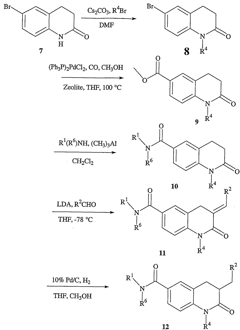
Scheme 2.
