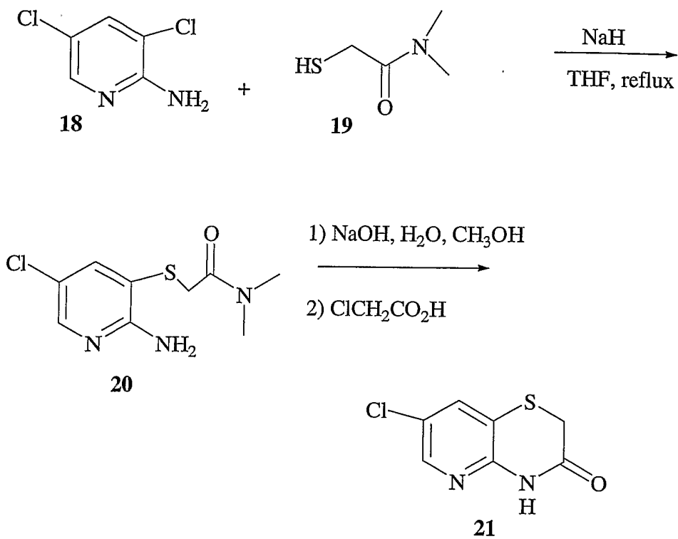
Scheme 3b.
