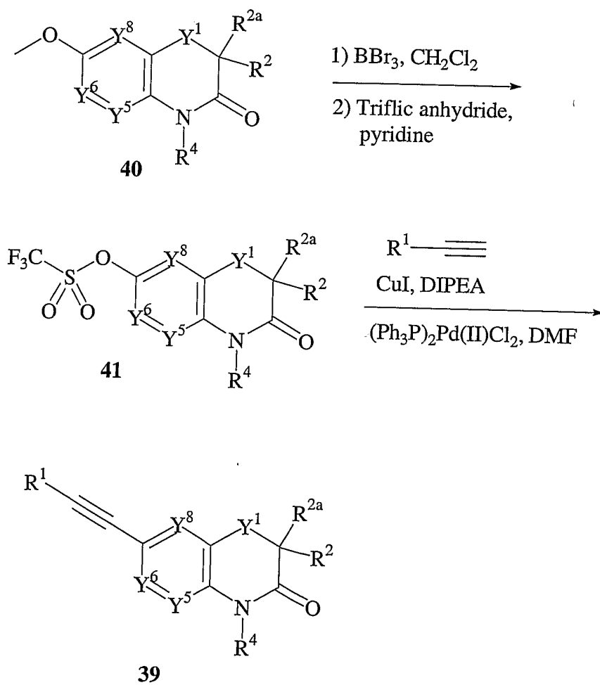
Scheme 5b.
