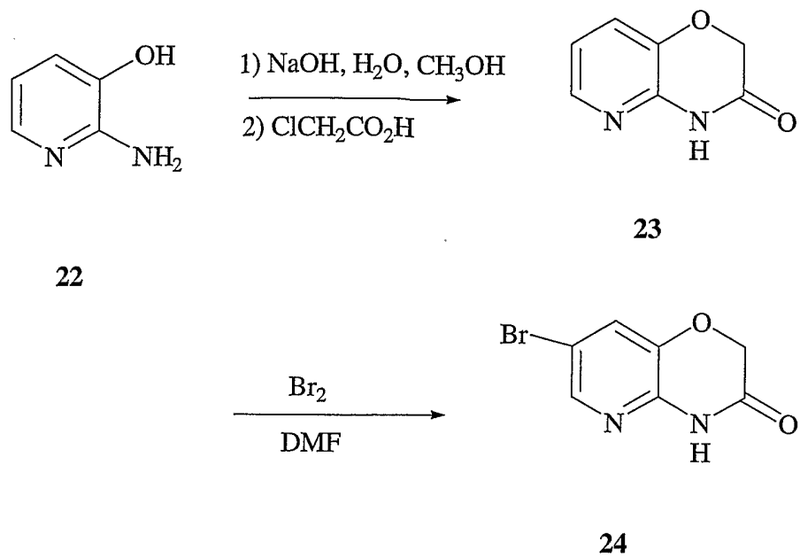
Scheme 3c.
