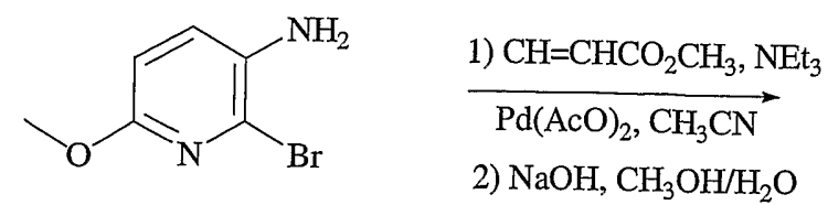
Scheme 4c.
