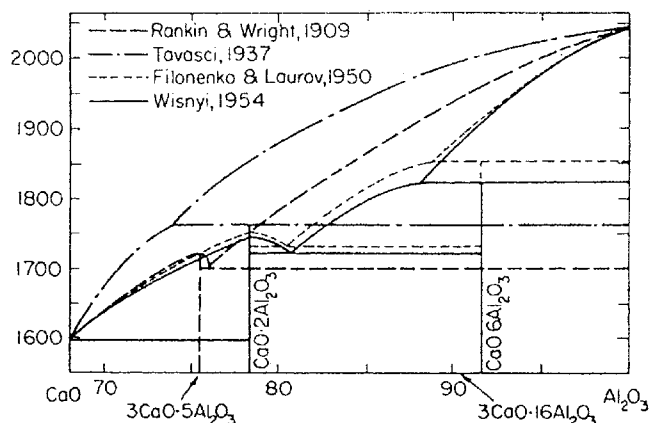
System CaO-Al 2 O 3 ; high alumina portion.
