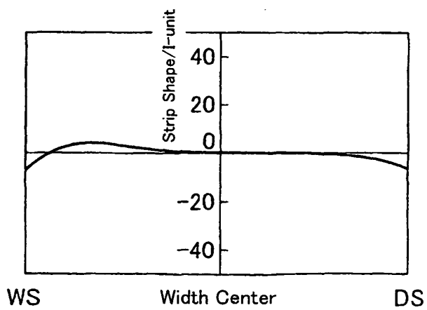
(c) Strip-Widthwise Distribution of Elongation difference
