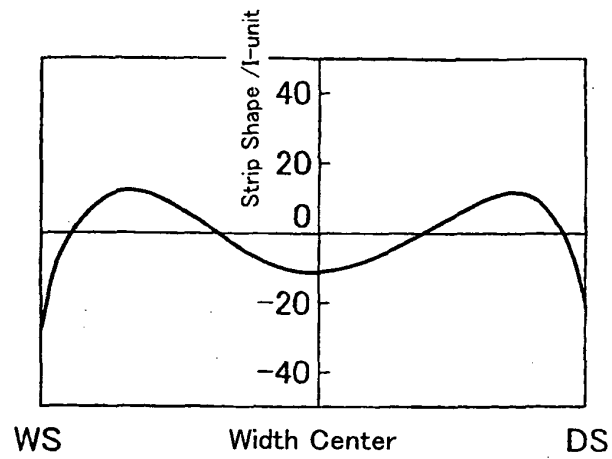
(a) Measurement Result of Shape Meter
