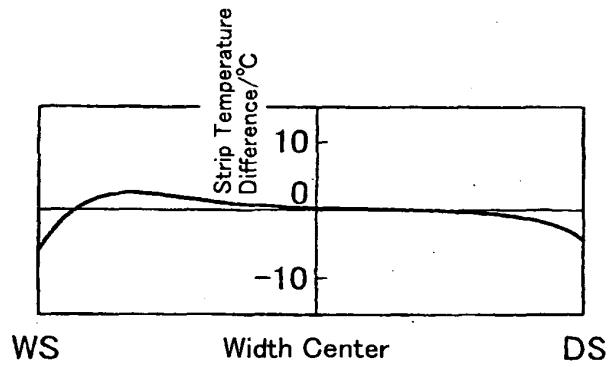
(b) Strip-Widthwise Temperature Distribution
