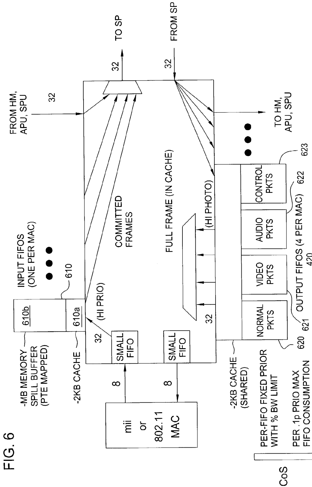
MI - MAC INTERFACE SUBUNIT
