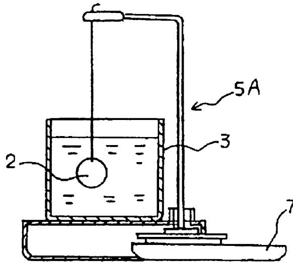
FIG. 8 (PRIOR ART)
