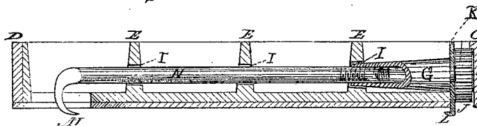
Figure 3. Section through P.S.
