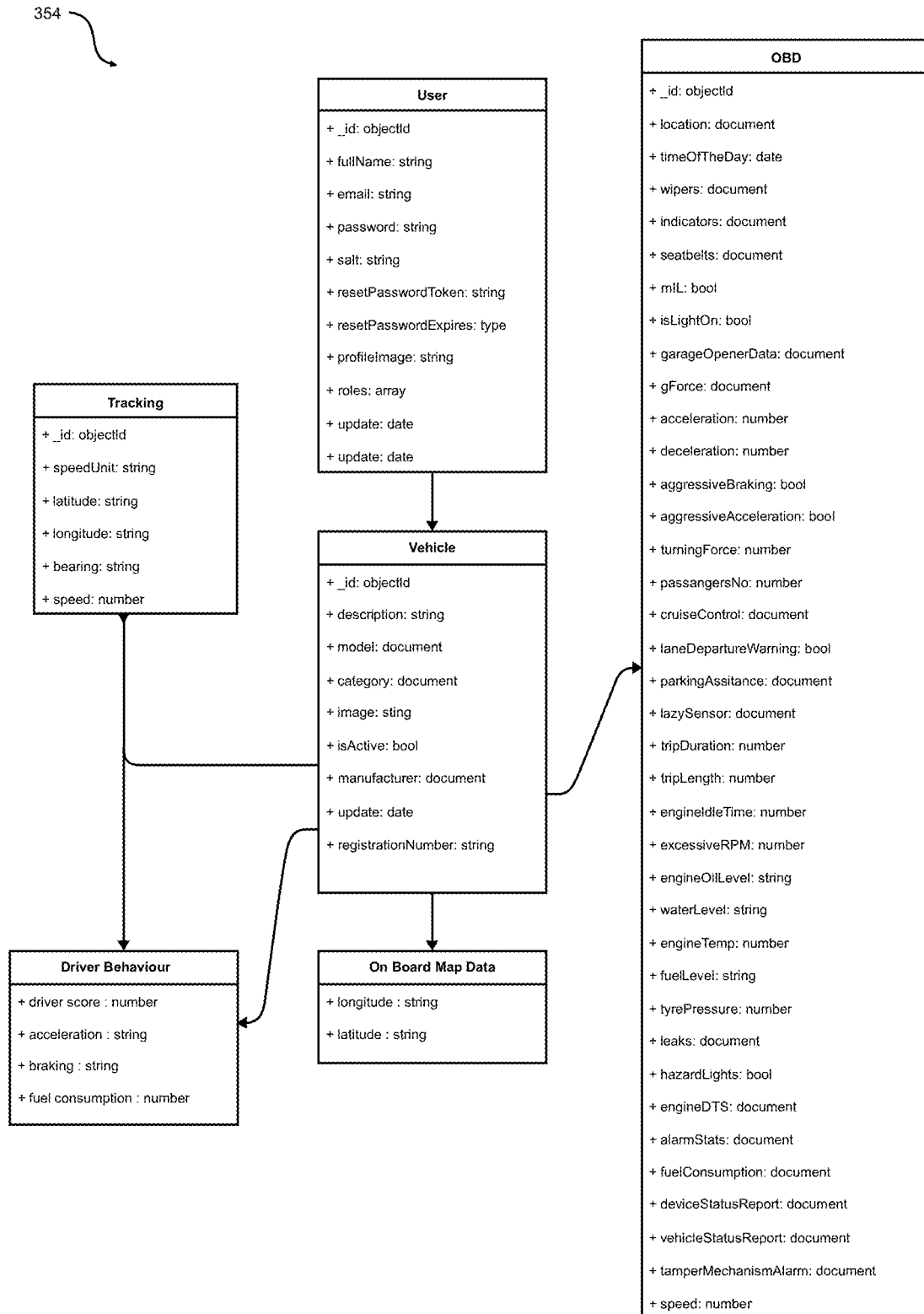
Figure 2(A) - System class diagram for tracking vehicle process
