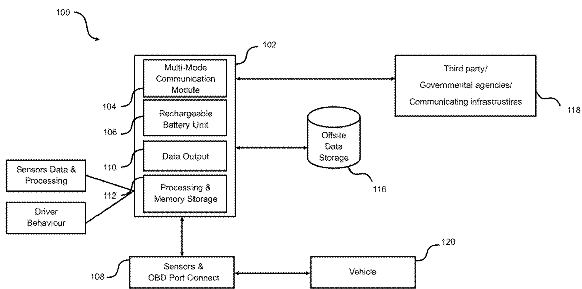
Figure 1: - Block Diagram of Technical Infrastructure
