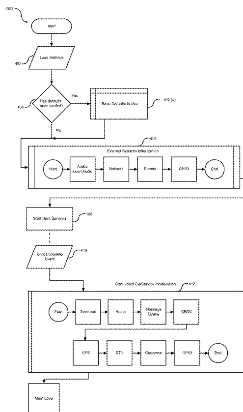
Initialization Process-Flow chart
