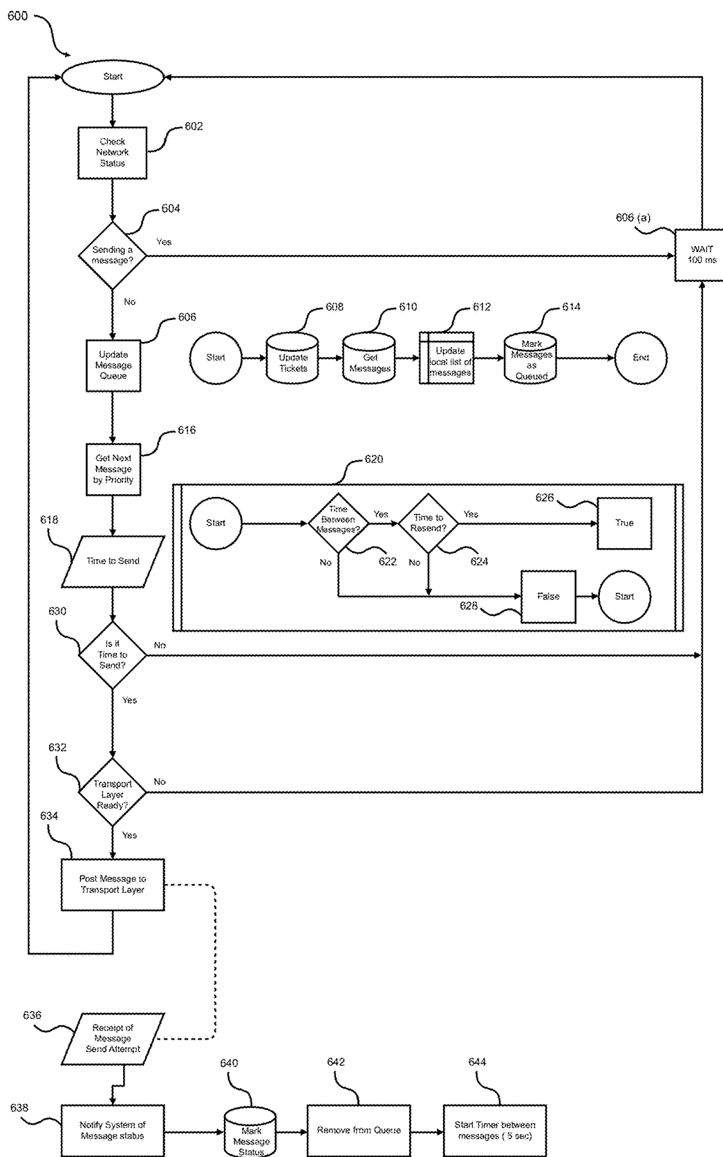
Figure 7 - Device Messaging Process
