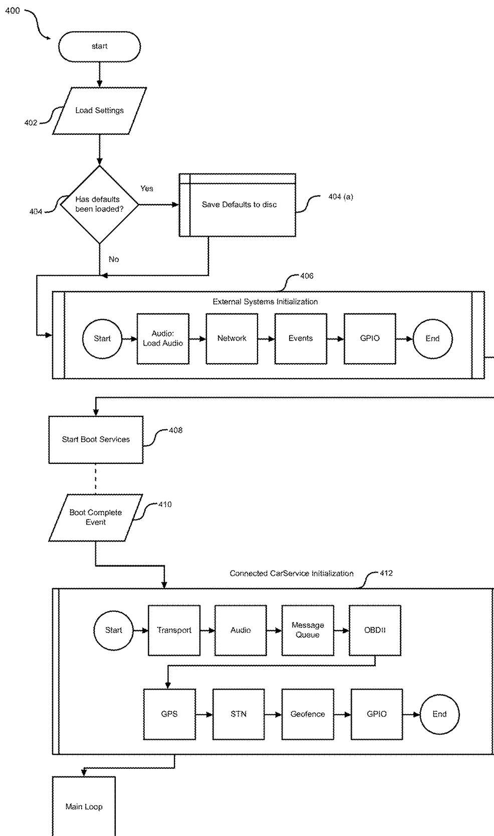
Figure 5: - Initialization Process-Flow chart
