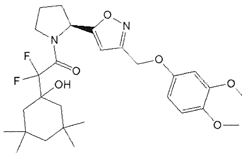
25 30 35 (S)-1-(2-(3-((3,4-Dimethoxyphenoxy)methyl)isoxazol-5-yl)pyrrolidin-1-yl)-2,2-difluoro-2-(1-hydroxy-3,3,5,5-tetramethylcyclohexyl)ethanone (Compound 10)
