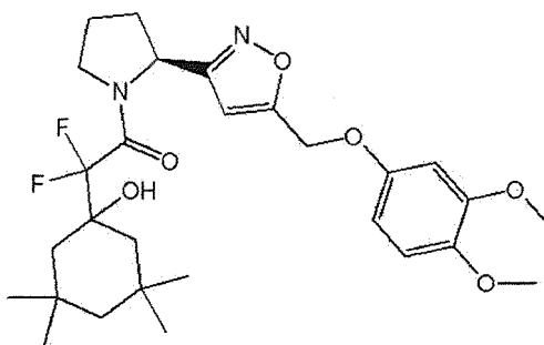
(S)-1-(2-(5-((3,4-Dimethoxyphenoxy)methyl)isoxazol-3-yl)pyrrolidin-1-yl)-2,2-difluoro-2-(1-hydroxy-3,3,5,5-tetramethylcyclohexyl)ethanone (Compound 1)
