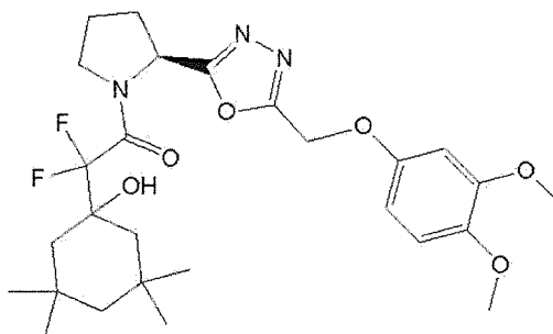
(S)-1-(2-(5-((3,4-Dimethoxyphenoxy)methyl)-1,3,4-oxadiazol-2-yl)pyrrolidin-1-yl)-2,2-difluoro-2-(1-hydroxy-3,3,5,5-tetramethylcyclohexyl)ethanone (Compound 2)
