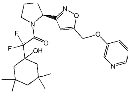
(S)-2,2-Difluoro-2-(1-hydroxy-3,3,5,5-tetramethylcyclohexyl)-1-(2-(5-((pyridin-3-yloxy)methyl)isoxazol-3-yl)pyrrolidin-1-yl)ethanone (Compound 40)
