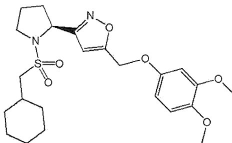
(S)-3-(1-((Cyclohexylmethyl)sulfonyl)pyrrolidin-2-yl)-5-((3,4-dimethoxyphenoxy)methyl)isoxazole (Compound 43)
