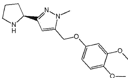
(S)-5-((3,4-Dimethoxyphenoxy)methyl)-1-methyl-3-(pyrrolidin-2-yl)-1H-pyrazole
