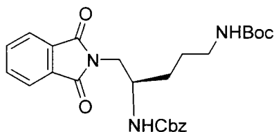
Benzyl tert-butyl (5-(1,3-dioxoisindolin-2-yl)pentane-1,4-diyl)(S)-dicarbamate
