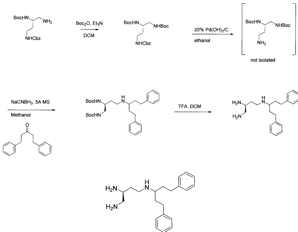
(S)-N 4 -(1,5-diphenylpentan-3-yl)butane-1,2,4-triamine 3 TFA
