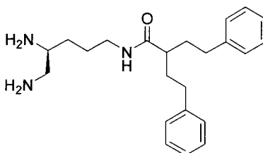
(S)-N-(4,5-Diaminopentyl)-2-phenethyl-4-phenylbutanamide
