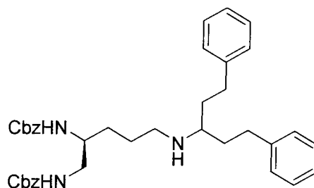
Dibenzy (5-((1,5-diphenylpentan-3-yl)amino)pentane-1,2-diyl)(S)-dicarbamate
