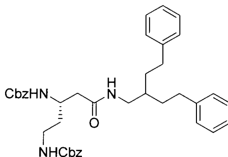
Dibenzyl (5-oxo-5-((2-phenethyl-4-phenylbutyl)amino)pentane-1,3-diyl)(S)-dicarbamate
