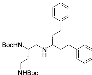
Benzyl tert-butyl (4-((1,5-diphenylpentan-3-yl)amino)butane-1,3-diyl)(S)-dicarbamate
