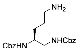
Dibenzy (5-aminopentane-1,2-diyl)(S)-dicarbamate
