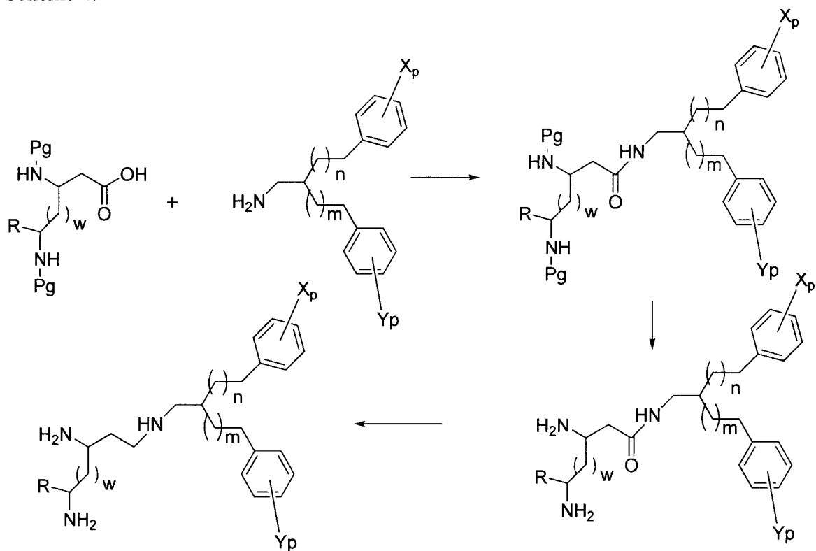
Scheme 4.
