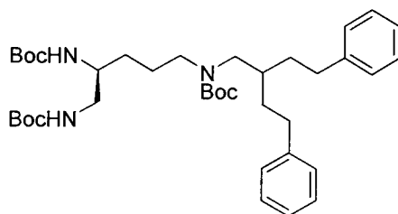
Di-tert-butyl (5-((tert-butoxycarbonyl)(2-phenethyl-4-phenylbutyl)amino)pentane-1,2-diyl)(S)-dicarbamate
