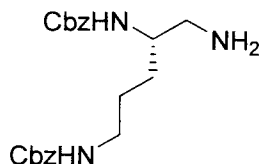
Dibenzy (5-aminopentane-1,4-diyl)(S)-dicarbamate
