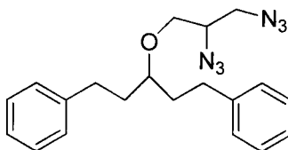
(3-(2,3-diazidopropoxy)pentane-1,5-diyl)dibenzene
