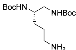
Di-tert-butyl (5-aminopentane-1,2-diyl)(S)-dicarbamate
