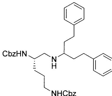
Dibenzy (5-((1,5-diphenylpentan-3-yl)amino)pentane-1,4-diyl)(S)-dicarbamate
