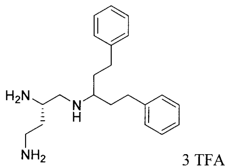
(S)-N 1 -(1,5-diphenylpentan-3-yl)butane-1,2,4-triamine 3TFA
