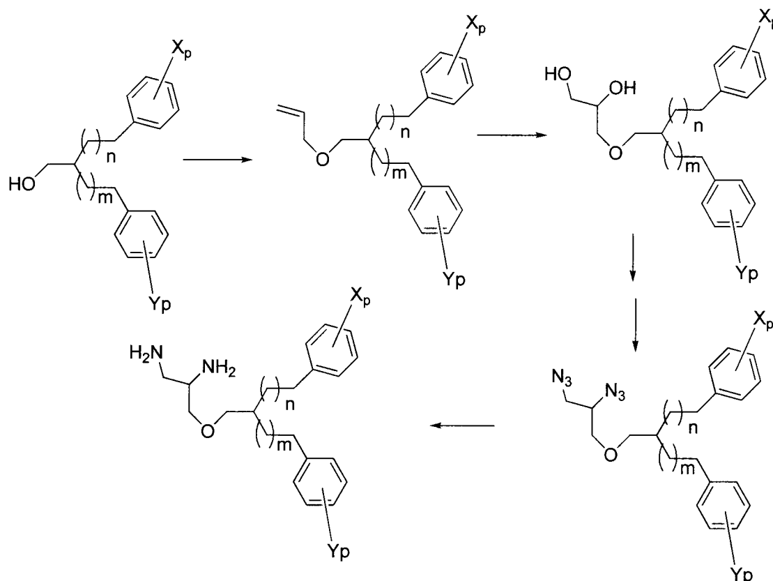
Scheme 8
