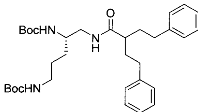
Di-tert-butyl (5-(2-phenethyl-4-phenylbutanamido)pentane-1,4-diyl)(S)-dicarbamate
