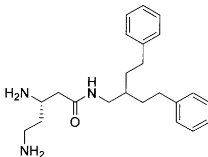
(S)-3,5-Diamino-N-(2-phenethyl-4-phenylbutyl)pentanamide
