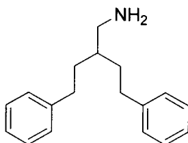
2-Phenethyl-4-phenylbutan-1-amine
