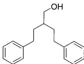
2-Phenethyl-4-phenylbutan-1-ol
