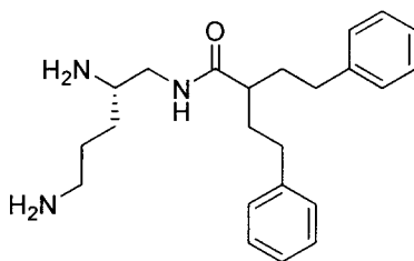
(S)-N-(2,5-Diaminopentyl)-2-phenethyl-4-phenylbutanamide
