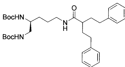
Di-tert-butyl (5-(2-phenethyl-4-phenylbutanamido)pentane-1,2-diyl)(S)-dicarbamate
