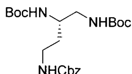
Benzyl di-tert-butyl butane-1,2,4-triyl(S)-tricarbamate
