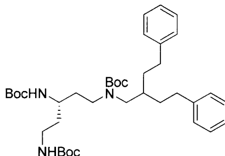
Di- t -butyl (5-(((tert-butoxycarbonyl)(2-phenethyl-4-phenylbutyl)amino)pentane-1,3-diyl) (S)-dicarbamate
