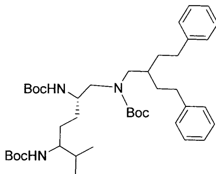
di- tert -butyl ((2 S )-1-(( tert -butoxycarbonyl)(2-phenethyl-4-phenylbutyl)amino)-6-methylheptane-2,5-diyl)dicarbamate
