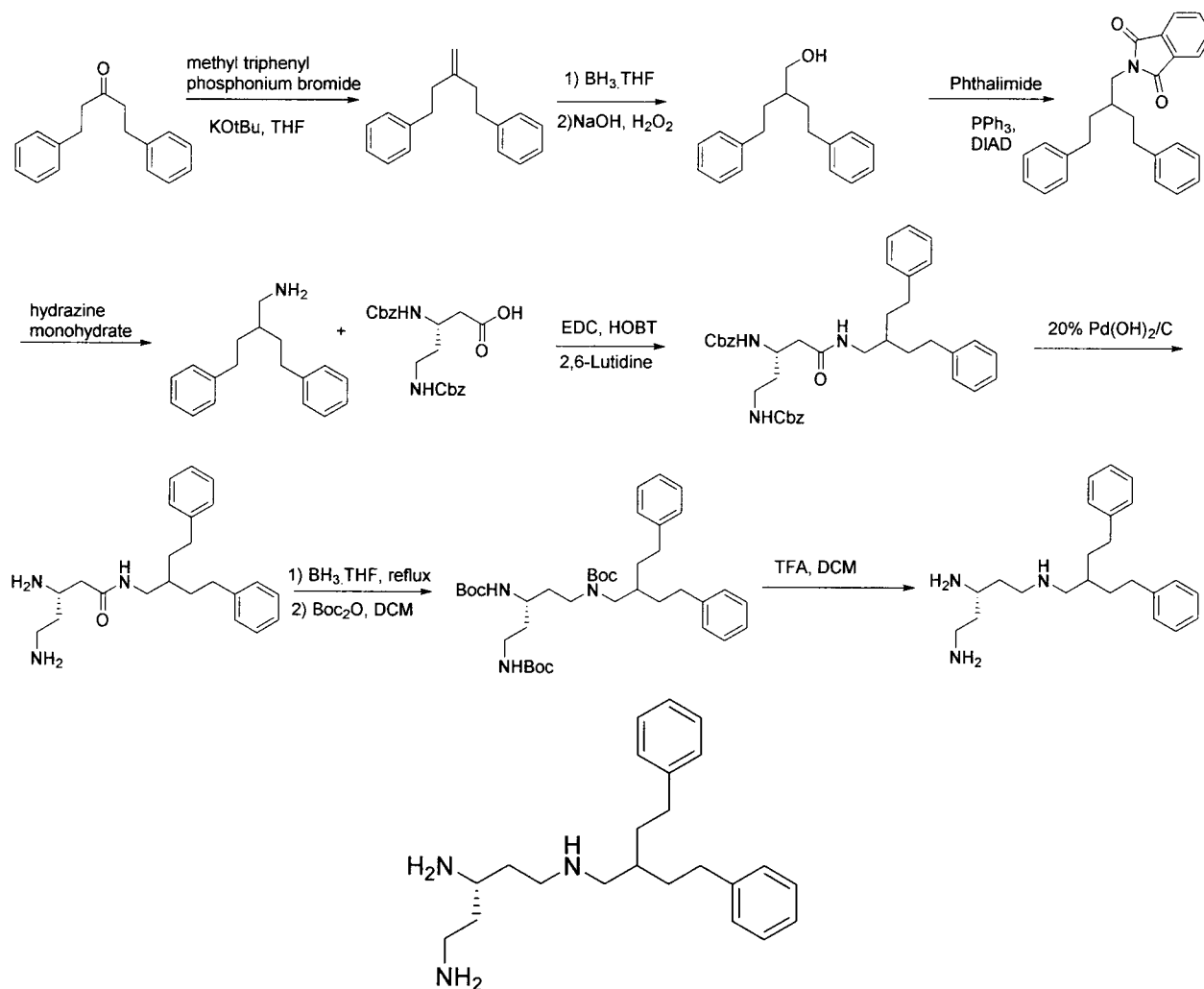
(S)-N 1 -(2-phenethyl-4-phenylbutyl)pentane-1,3,5-triamine 3 TFA
