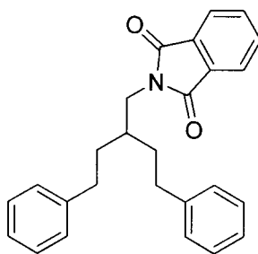
2-(2-Phenethyl-4-phenylbutyl)isoindoline-1,3-dione
