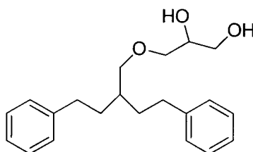
3-(2-phenethyl-4-phenylbutoxy)propane-1,2-diol
