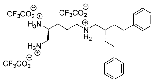
(S)-N 5 -(2-phenethyl-4-phenylbutyl)pentane-1,2,5-triaminium 2,2,2-trifluoroacetate
