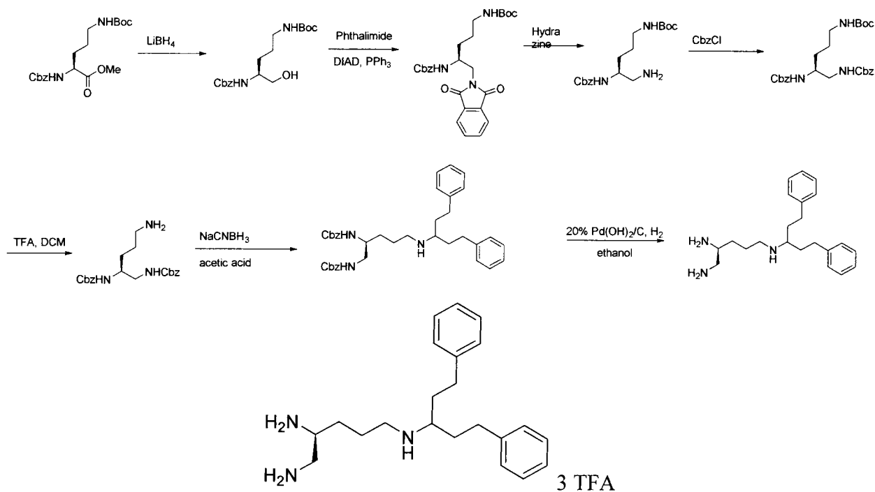
(S)-N 5 -(1,5-diphenylpentan-3-yl)pentane-1,2,5-triamine 3 TFA
