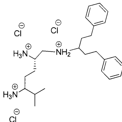
(2S)-N 1 -(1,5-diphenylpentan-3-yl)-6-methylheptane-1,2,5-triaminium chloride
