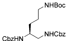
Dibenzyl tert-butyl pentane-1,2,5-triyl(S)-tricarbamate
