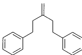
(3-Methylenepentane-1,5-diyl)dibenzene
