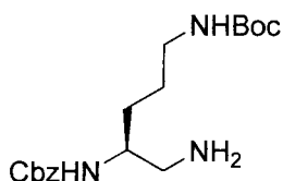
Benzyl tert-butyl (5-aminopentane-1,4-diyl)(S)-dicarbamate
