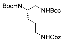
Benzyl di-tert-butyl pentane-1,2,5-triyl(S)-tricarbamate
