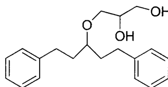
3-((1,5-diphenylpentanyl)oxy)propane-1,2-diol
