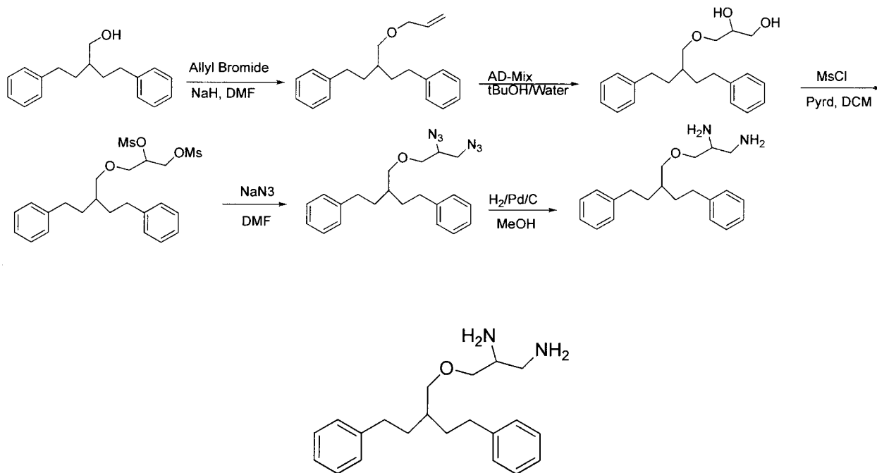
3-(2-phenethyl-4-phenylbutoxy)propane-1,2-diamine
