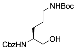
Benzyl tert-butyl (5-hydroxypentane-1,4-diyl)(S)-dicarbamate
