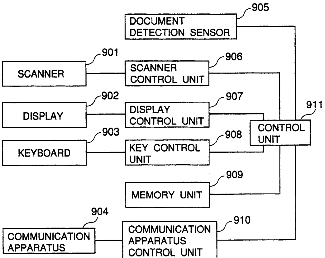
FIG. 11 PRIOR ART
