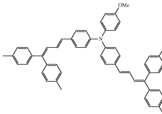
Charge transporting material A1
