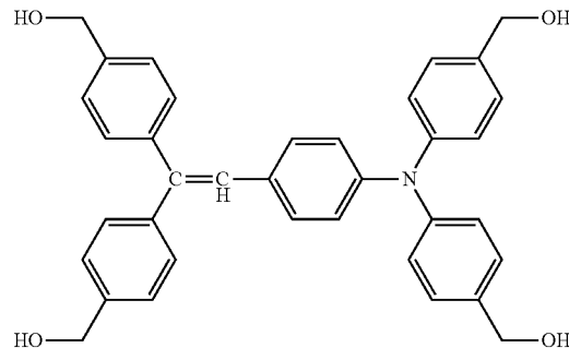
Charge transporting material B1
