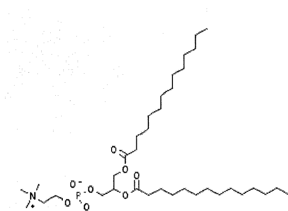
Dimyristoyl-phosphatidylcholine or DMPC
