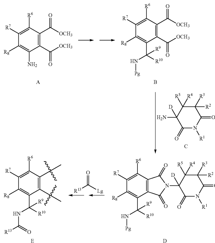
Scheme 1
