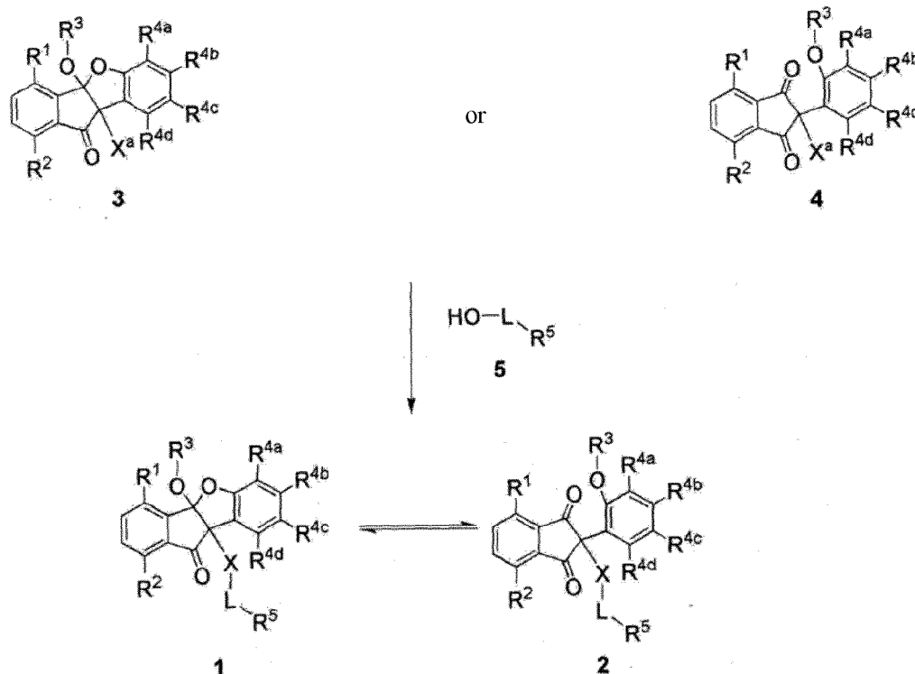
[Reaction Equation 1]
