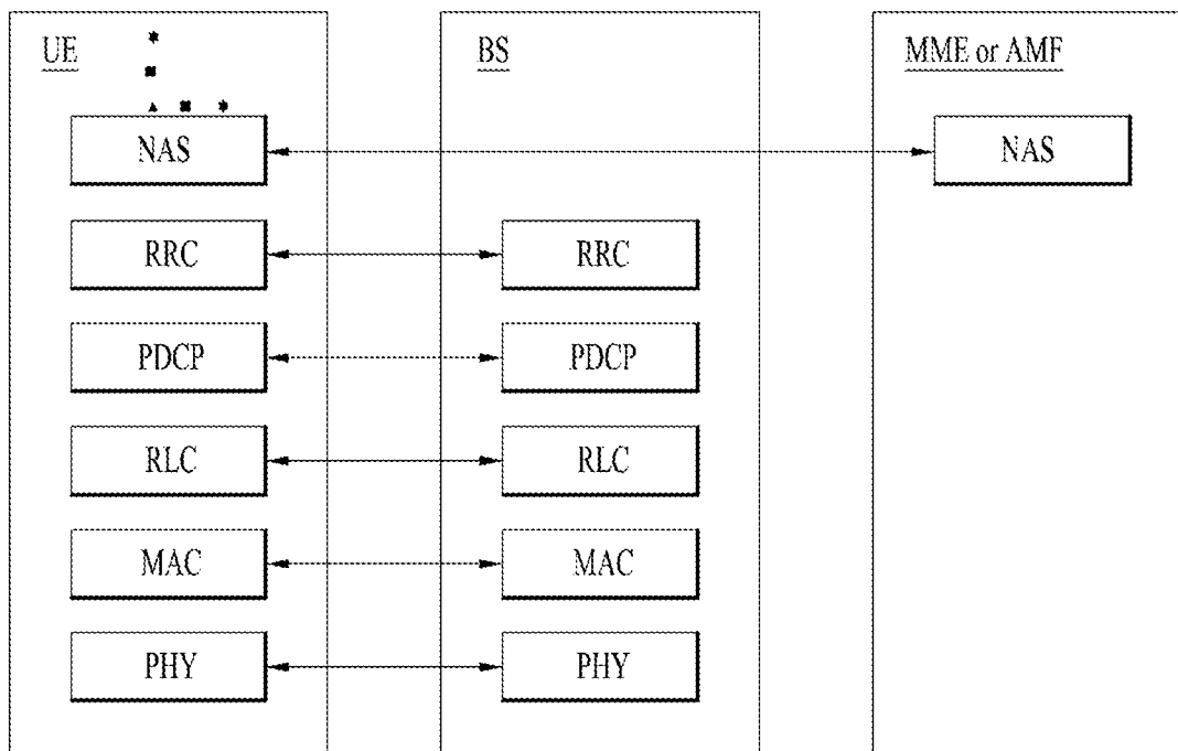
Control Plane Protocol Stack
