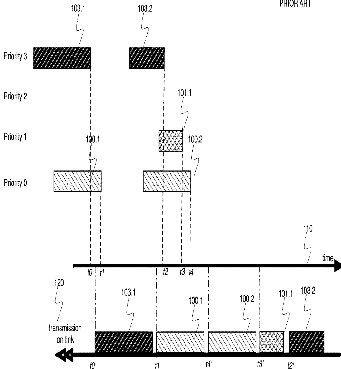
Figure 1 PRIOR ART
