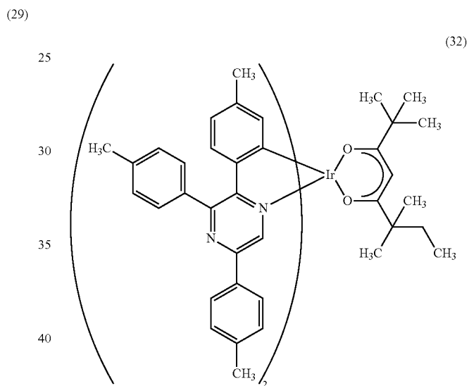
[Chemical Formula 14]
