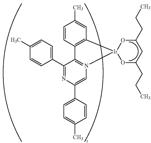
[Chemical Formula 13]
