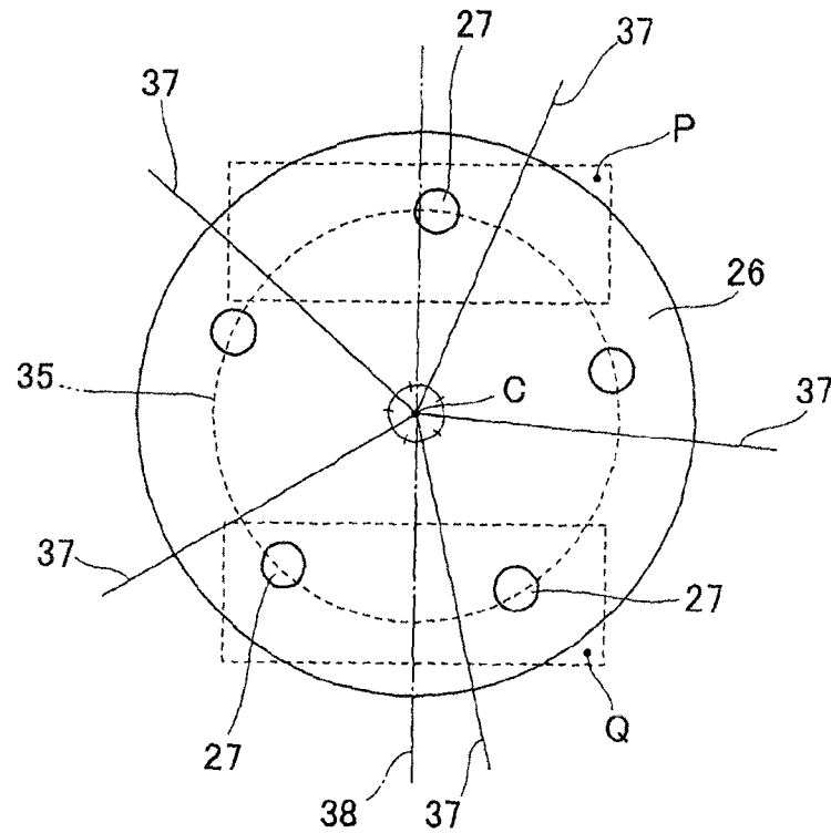
FIG. 13 (PRIOR ART)
