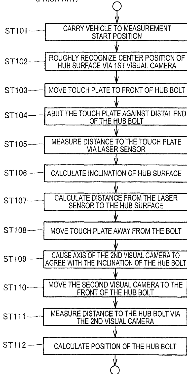
FIG. 14 (PRIOR ART)
