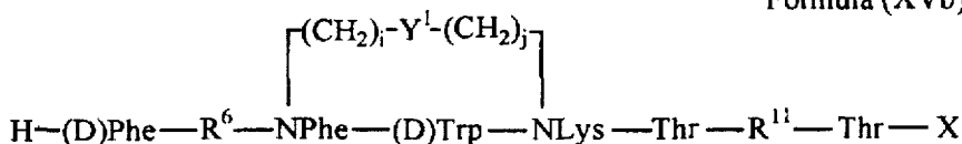
Formula (XVb)
