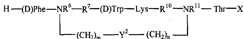
Formula (XIVb)
