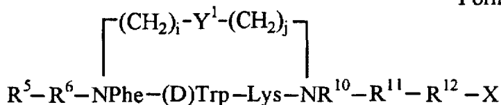
Formula (XVIa)
