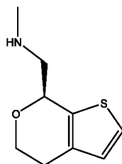
(S)-TPMA.
