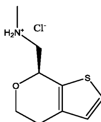
(S)-TPMA HCl
