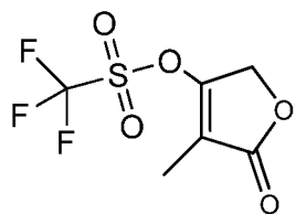
4-Methyl-5-oxo-2,5-dihydrofuran-3-yl trifluoromethanesulfonate
