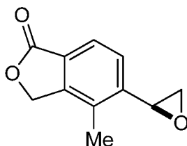
4-methyl-5-[(2S)-oxiran-2-yl]-2-benzofuran-1(3H)-one
