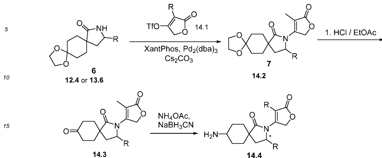
SCHEME 14
