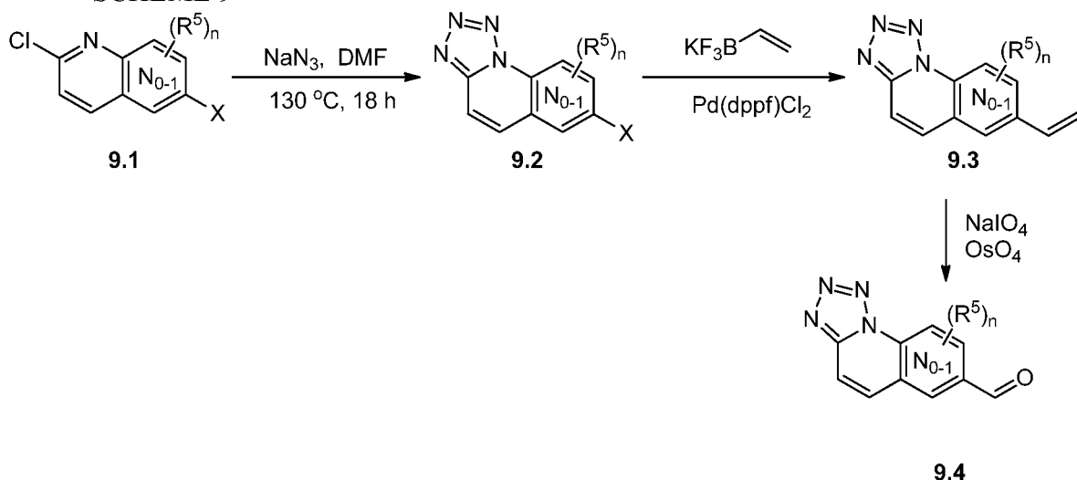
SCHEME 9
