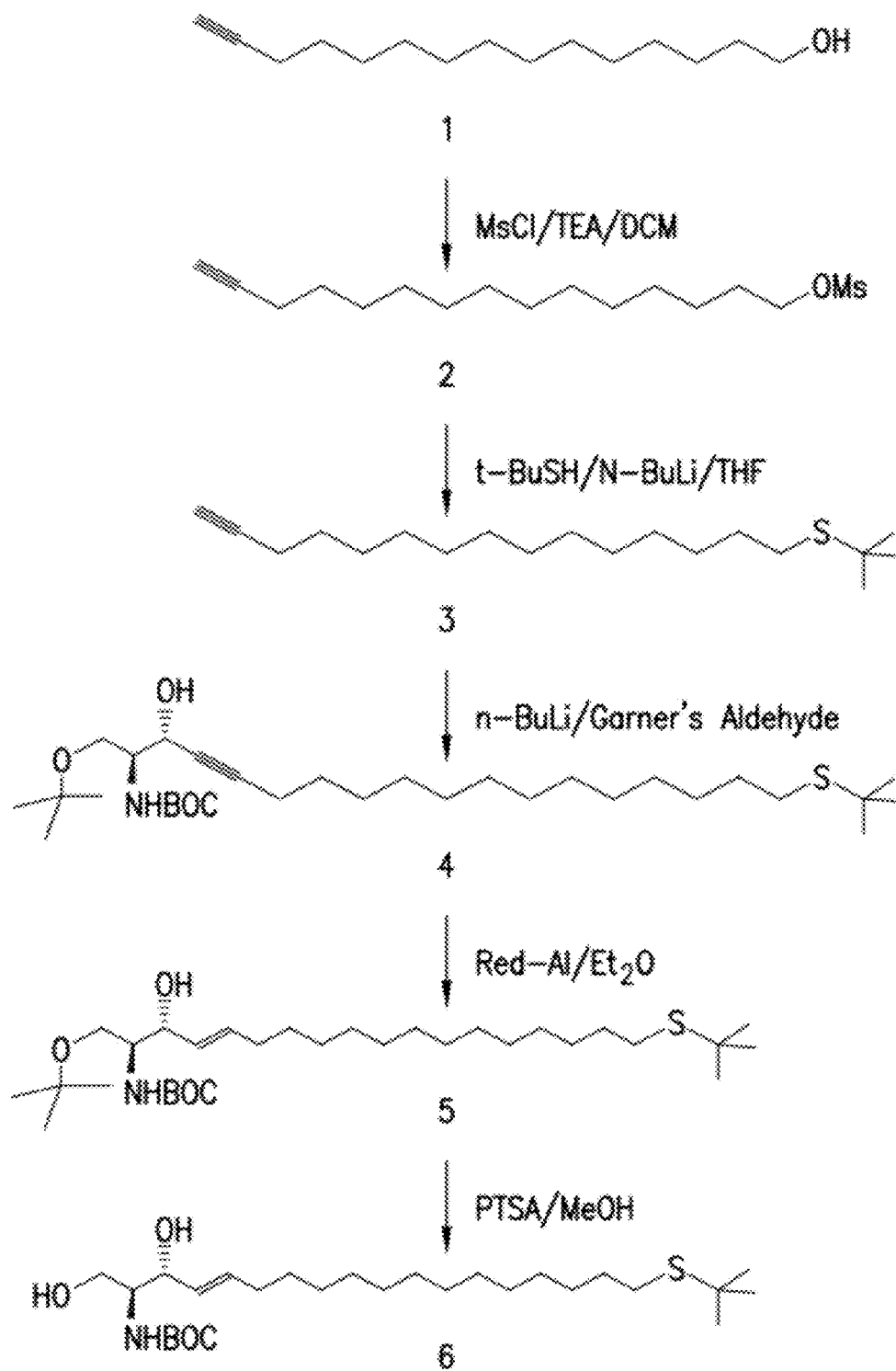
Synthesis of Typical Thiolated S1P-Related Antigen
