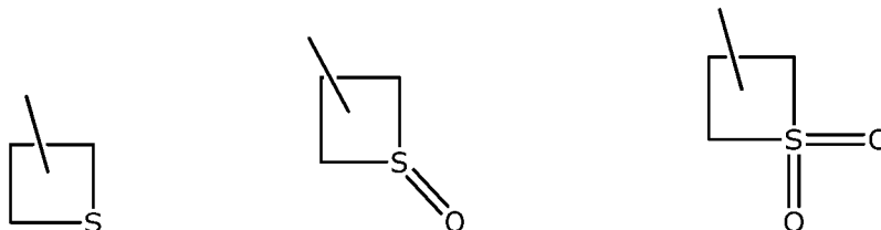
thietanyl
