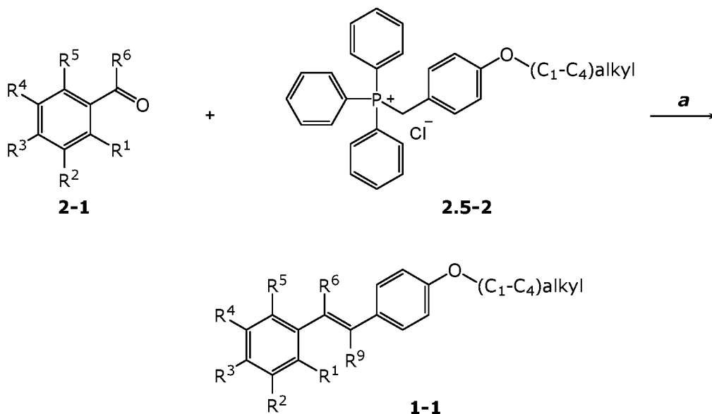
Scheme 2.5
