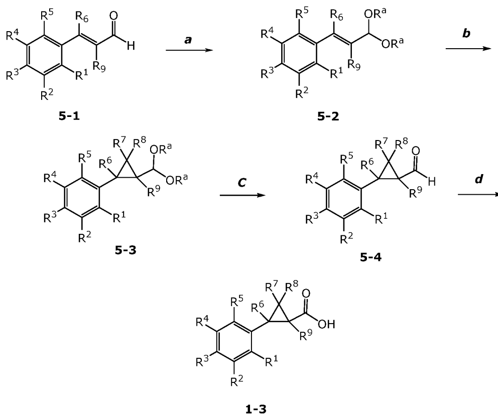
Scheme 5
