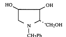
1,4-Dideoxy-1,4-benzylimino-L-ribitol
