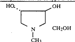
1,4-Dideoxy-1,4-imino-[N-methyl]-L-arabinitol
