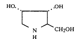
1,4-Dideoxy-1,4-imino-D-ribitol
