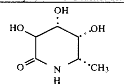
1,5-Dideoxy-1,5-imino-L-fuconolactam
