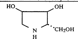
1,4-Dideoxy-1,4-imino-L-ribitol
