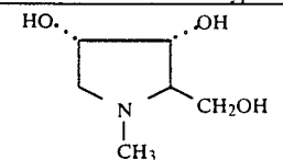
1,4-Dideoxy-1,4-imino-[N-methyl]-D-ribitol
