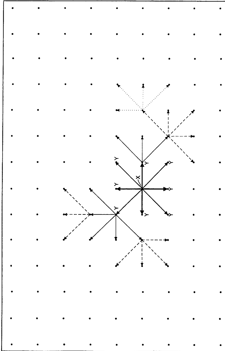
FIG. 2 SHOWS SCHEMATIC VIEW OF COLONY GROWTH
