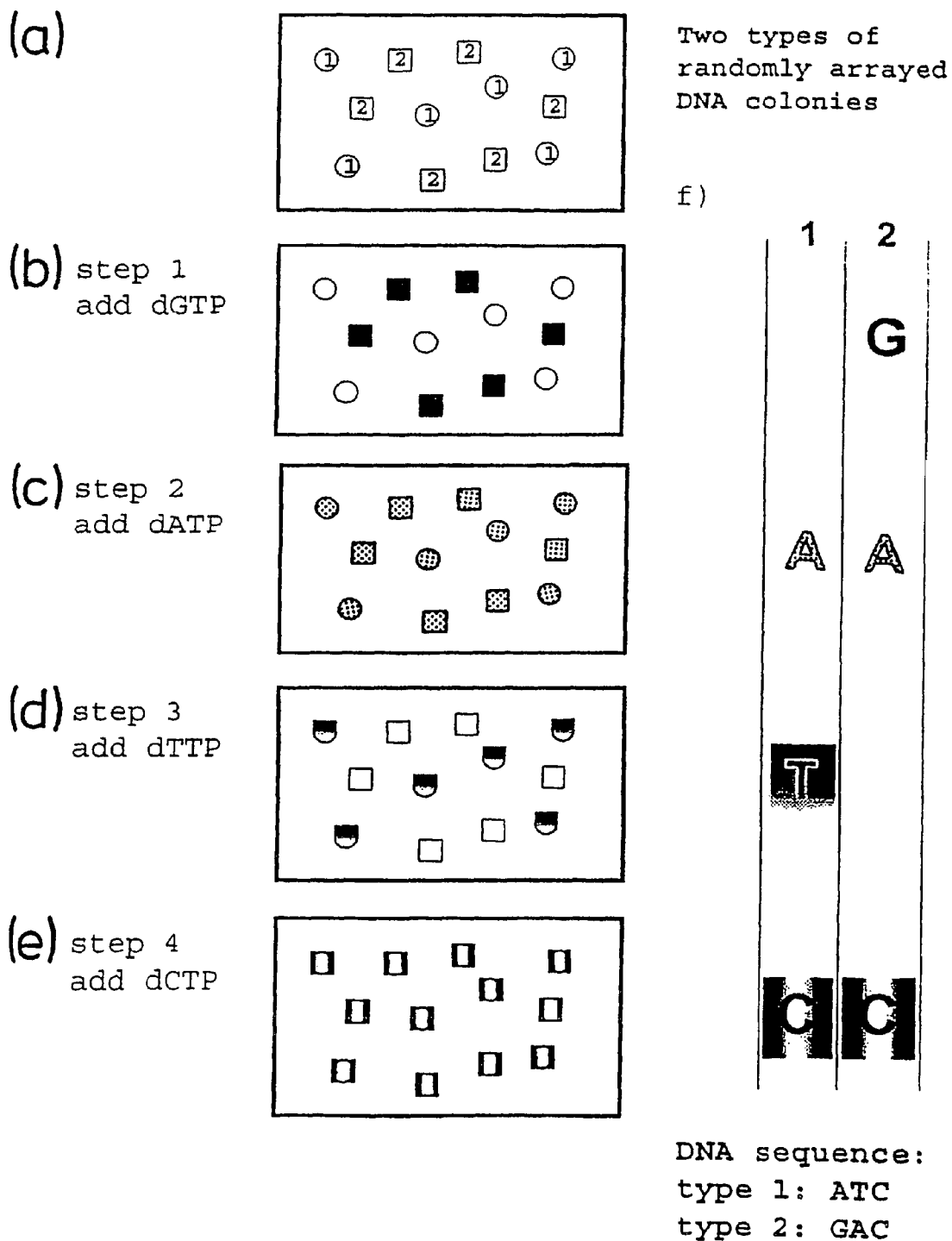
FIG. 17 in situ Sequencing
